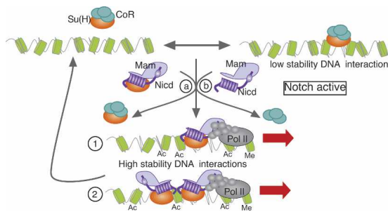
Figure 5. Dynamic model for Su(H) recruitment. Fast exchange and low residency of Su(H) (orange) when complexed with corepressors (turquoise). Following Notch activation, Su(H) complex with Nidc (dark purple) and Mam (light purple) is more stably associated with the DNA, possibly due to (1) interactions with other factors (gray, Pol II and associated factors) and/or (2) cooperative binding. This is accompanied by nucleosome (green) loss and histone modifications (Ac, me). Su(H) may form a complex with Nidc and Mam prior to DNA binding (a) or exchange could occur on transiently bound Su(H) (b). After recruitment, Nidc is subsequently modified and most likely degraded (Fryer et al. 2004), so Su(H) reverts to a lower occupancy state.
