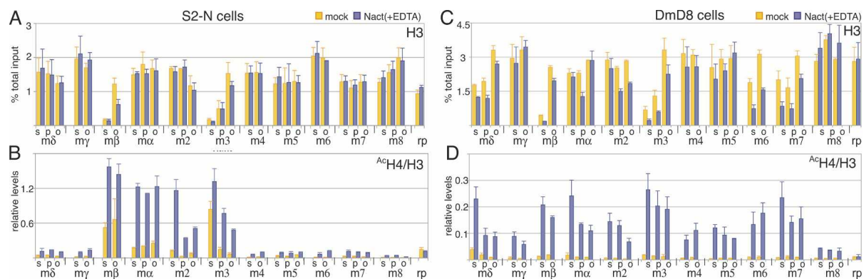
Figure 4. Chromatin modifications across E(spl) genes before and after Notch activation in S2-N and DmD8 cells. ChIP was performed with the indicated antibodies in S2-N (A,B) and DmD8 (C,D) cells before (orange) and 25 min after (blue) EDTA and bound fragments were quantified by real-time PCR. Results are an average of three independent experiments (error bars indicate standard error of the mean). (B,D) For each column, levels were first calculated relative to input and then as a ratio to the equivalent sample from the α-H3 ChIP. Controls were rp49 (rp). In α-H3 ChIP, the decrease in enrichment of mβ -o ( P = 0.02 ) and m3 -o ( P = 0.05 ) in S2-N cells and of mδ -s ( P = 0.006 ), mδ -p ( P = 0.03 ), mβ -s ( P = 0.002 ), mα -p ( P = 0.02 ), m2 -p ( P = 0.008 ), m3 -s ( P = 0.03 ), m3 -p ( P = 0.03 ), m6 -s ( P = 0.004 ), and m7 -s ( P = 0.03 ) in DmD8 cells are all significant.
