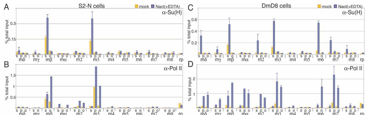
Figure 2. Su(H) occupancy increases after Notch activation. ChIP with \alpha -Su(H) (A,C) or \alpha -Pol II (phosphorylated CTD) (B,D) antibodies in S2-N (A,B), and DmD8 (C,D) cells before (orange) or 30 min after (blue) EDTA. Precipitated DNA was quantified by real-time PCR. Each gene is represented by two or three fragments. (s) Su(H)-binding/enhancer region; (p) promoter; (o) ORF. A single 5' region was amplified when Su(H) sites were close to the promoter. Control was rp49 (rp). Results are average of three independent experiments (error bars indicate standard error of the mean). Increase in enrichment after activation of mβ -s ( P = 0.03 ) and m3 -s ( P = 0.04 ) in S2-N cells and of mδ -s ( P = 0.04 ), mβ -s ( P = 0.04 ), m3 -s ( P = 0.003 ), m6 -s ( P = 0.002 ), and m7 -s ( P = 0.02 ) in DmD8 cells is significant.
