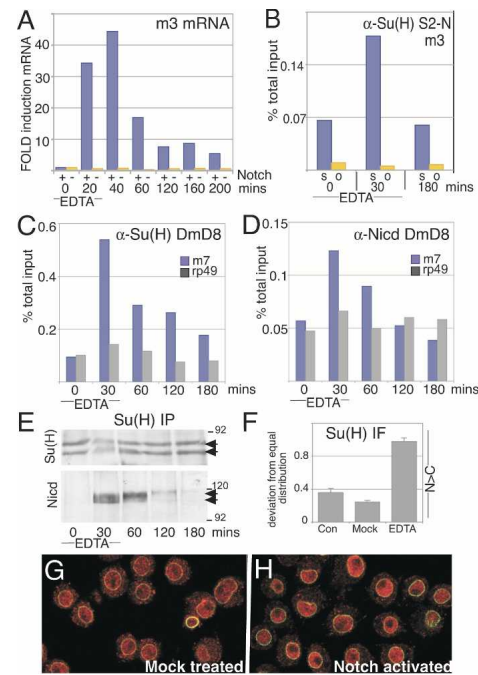
Figure 3. Time course of Su(H) occupancy and Nidc recruitment. (A) m3 mRNA levels in S2-N (blue) and S2 cells (orange) at the indicated times relative to EDTA treatment. (B–D) α-Su(H) (B,C) or α-Nidc (D) ChIP at the indicated times relative to EDTA treatment in S2-N (B) or DmD8 (C,D) cells. Enrichment of m3 enhancer (blue) and ORF (orange) (B) or m7 enhancer (blue) and rp49 ORF (control, gray) (C,D) were quantified. (E) Su(H) was immunoprecipitated at the indicated times and immunoprecipitates were probed to detect Su(H) (top panel, arrows) or Nidc (bottom panel, arrows). Approximate positions of molecular weight markers (in kilodaltons) are indicated. (F–H) Su(H) immunofluorescence (IF) (α-Su(H), red) (G,H) in S2-N cells treated as indicated. In F, distribution was quantified as described in the Supplemental Material. Differences between EDTA and control or mock cells were significant ( P < 0.001 ) in S2-N cells. α-DMO (green) marks the nuclear envelope in G and H.
