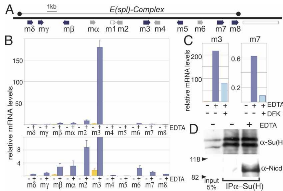
Figure 1. EDTA elicits Notch activation in S2-N cells. (A) Diagram of E(spl) complex. Genes are indicated by arrows: basic helix-loop-helix genes (blue); Bearded-type (gray); not Notch responsive (white). (B) mRNA levels of E(spl) genes before and 30 min after EDTA treatment of S2-N cells. Bottom panel shows results plotted on a more sensitive scale. (C) m3 and m7 RNA levels in EDTA-treated S2-N cells \pm \gamma -secretase inhibitor DFK-167 (300 \mu M). (D, top panel) Su(H) is detected as two bands in the total input and in \alpha -Su(H) immunoprecipitates with and without EDTA treatment. (Bottom panel) Nicd is only present in the immunoprecipitated sample from EDTA-treated cells. Positions of molecular weight markers (in kilodaltons) are indicated for the bottom panel.
