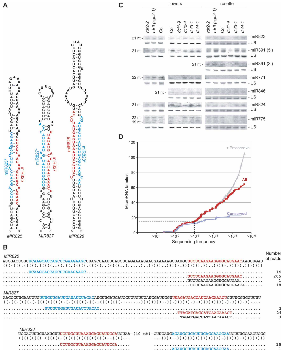
Figure 1. Newly identified Arabidopsis miRNAs. (A) Predicted secondary structures of miRNA hairpins highlighting the miRNA (red) and miRNA* (blue). (B) The miRNA hairpins of A, shown in bracket notation with a tally of reads mapping to the hairpin and nucleotides colored as in A. (C) RNA blots demonstrating that accumulation of six detectable miRNAs depended on DCL1, not DCL2, DCL3, DCL4, RDR2, or RDR6. As a loading control, blots were stripped and reprobed for U6. (D) Sequencing frequencies of Arabidopsis miRNA families. Shown are cumulative plots for all Arabidopsis miRNA families (red squares), conserved families (violet diamonds), and all families plus the 40 sequenced candidates (gray triangles). Fourteen families, 11 of which were conserved, were sequenced at a frequency of greater than one per 1000 (dashed line).
