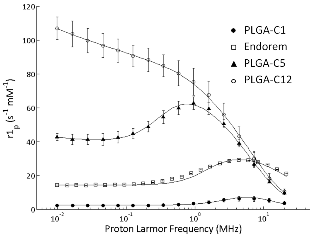
Figure 3. Profiles of 1/T_1 ^1\text{H} -NMRD (25°C and pH=7.4) of PLGA-Fe-NPs loaded with the different magnetic nanoparticles: C12 ( \circ ), C5 ( \blacktriangle ), Endorem ( \square ), and C1 ( \bullet ). The solid lines between data
