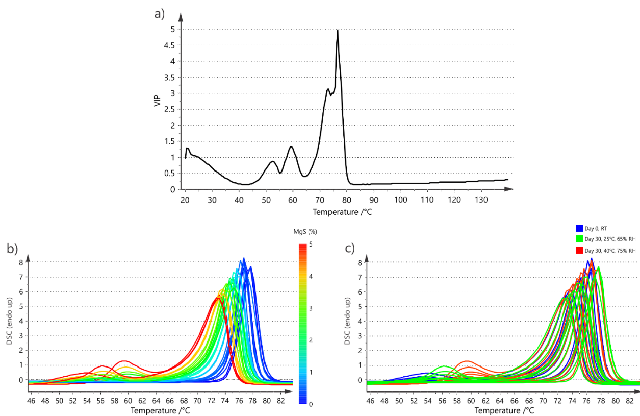
Figure S2. VIP plot of the DSC curves PLS model (a), DSC curves colored according to the MgS content (b) and stress conditions (c)
