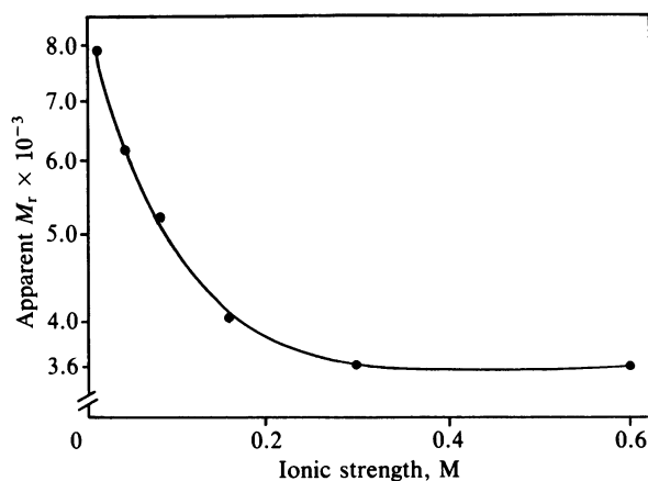
FIG. 3. Dependence on the ionic strength of the apparent molecular weight of phytochelatin, as determined by gel filtration.
