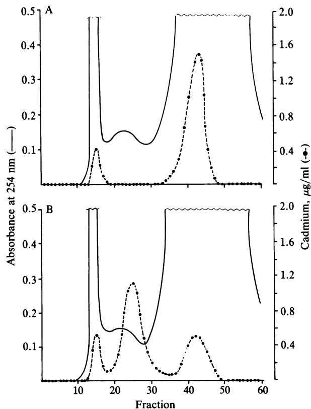
FIG. 1. Elution profiles of crude extracts from leaves of B. oleracea grown in the absence (A) or presence (B) of 90 \mu\text{M} \text{Cd}(\text{NO}_3)_2 . Prior to Sephadex G-50 gel filtration, \text{Cd}(\text{NO}_3)_2 was added to homogenates of untreated plants (A).
