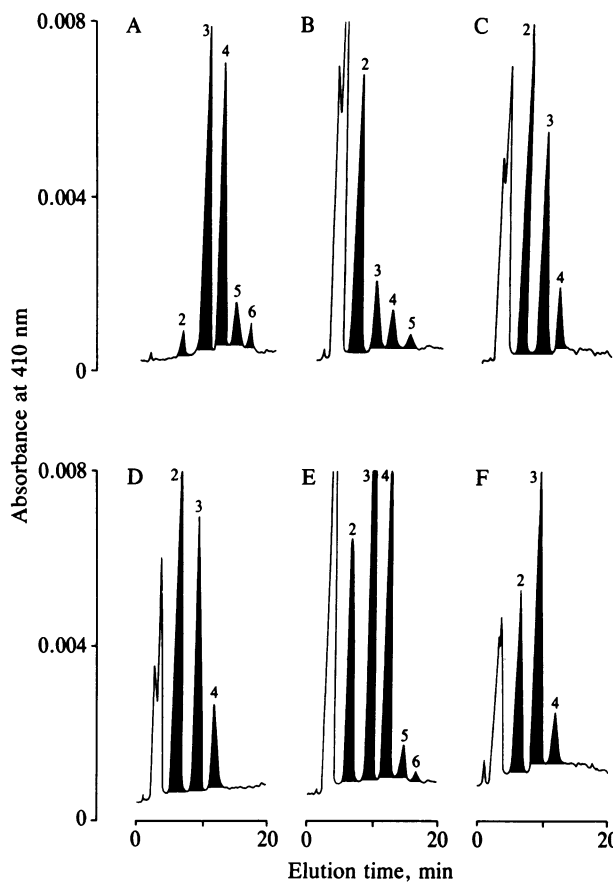
FIG. 2. Chromatogram of sulfhydryl-containing material from \text{Cd}^{2+} -exposed plants. Purified phytochelatin isolated from leaves of B. oleracea (A) was analyzed by HPLC, as well as crude extracts from cell suspension cultures of S. cucubalus (B) and A. tenuis (C) and from roots of Z. mays (D), L. esculentum (E), and E. crassipes (F). For A and E, plants were treated for 3 weeks with 90 \mu\text{M} \text{Cd}(\text{NO}_3)_2 , according to Wagner (13), whereas the other tissues were exposed for 3 days to 20 \mu\text{M} \text{Cd}(\text{NO}_3)_2 . The peaks corresponding to the individual phytochelatin are shaded and are identified by index number ( n , the number of \gamma -glutamylcysteine units). The unshaded double peak corresponds to cysteine, which was eluted at a lower retention time, and glutathione. Samples from plants not exposed to \text{Cd}^{2+} contained either no phytochelatin or only negligible quantities ( A_{410} < 0.0005 in this assay).
