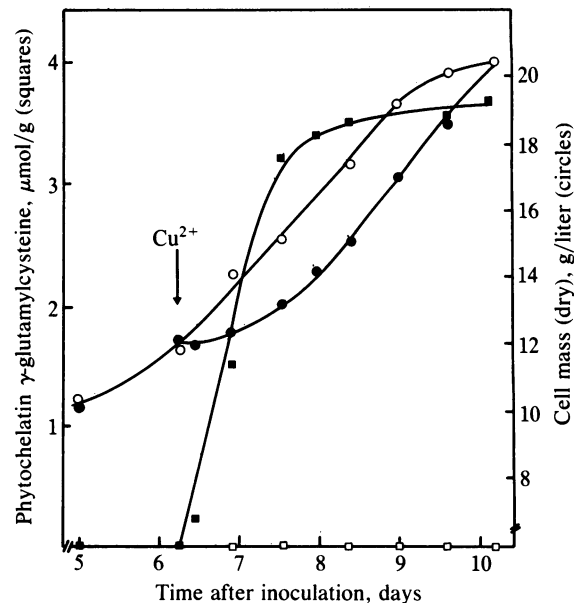
FIG. 6. Growth retardation and phytochelatin synthesis of R. serpentina cells during heavy metal stress. After administration of 50 \mu\text{M} \text{CuSO}_4 , phytochelatin was formed ( \blacksquare ); in nontreated cells, no phytochelatin was identified ( \square ). Growth of \text{Cu}^{2+} -treated cells ( \bullet ) was inhibited compared to the control ( \circ ).
