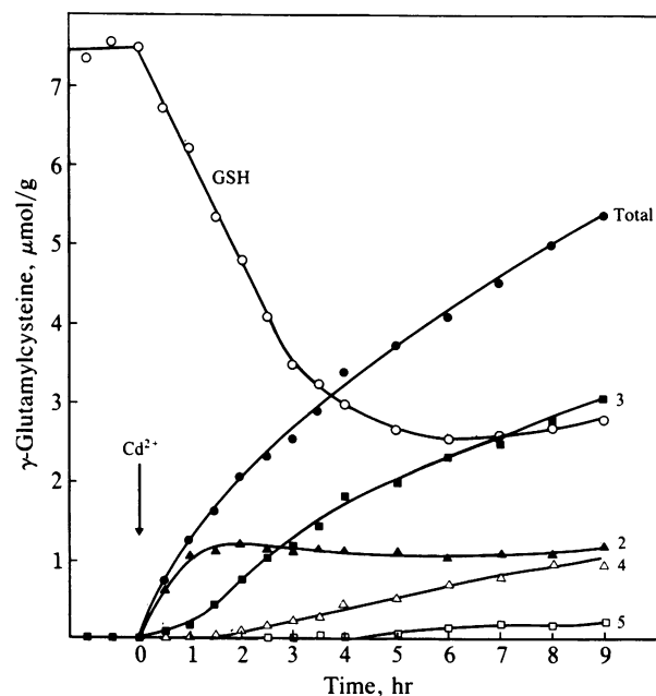
FIG. 4. Time course of phytochelatin induction and glutathione consumption after administration of 200 μM Cd(NO 3 ) 2 to R. serpentina cell suspension culture. Quantities of glutathione (GSH, ○), total phytochelatin (●), and individual phytochelatin with n (no. of γ-glutamylcysteine units per molecule) = 2 (▲), 3 (■), 4 (△), or 5 (□) are expressed as μmol of γ-glutamylcysteine per g (dry weight) of cells.
