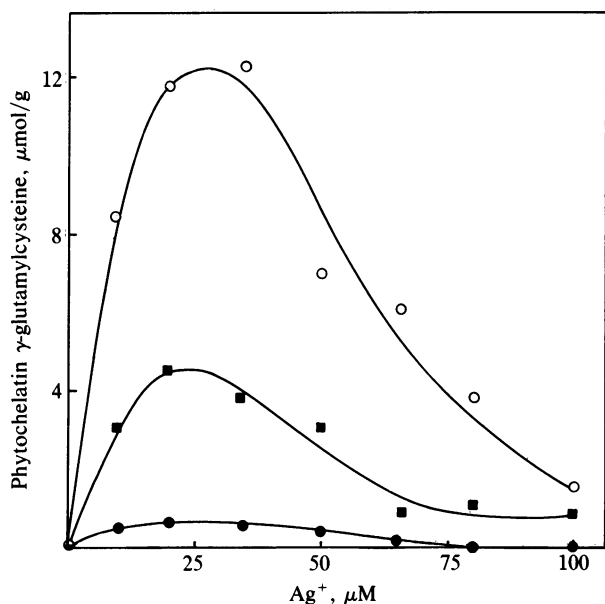
FIG. 5. Inhibition of phytochelatin synthesis by buthionine sulfoximine. R. serpentina cells were exposed to \text{AgNO}_3 6 hr after addition of buthionine sulfoximine, a specific inhibitor of the first enzyme of glutathione biosynthesis. After 3 days, the level of phytochelatin (expressed as \mu\text{mol} of \gamma -glutamylcysteine per g of dry weight) was determined in control cells ( \circ ) without inhibitor and in cells incubated in medium containing 0.2 mM ( \blacksquare ) or 2 mM ( \bullet ) inhibitor. Growth of cells not exposed to \text{Ag}^+ was not affected by buthionine sulfoximine.
