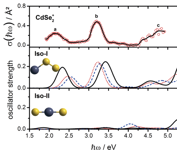
FIG. 6. Experimental CdSe 2 + absorption cross section \sigma(\hbar\omega) data points (red circles) and a 5-pt adjacent average as a guide to the eye (solid black line) compared to the optical absorption of Iso-I and Iso-II, calculated with EOM-CCSD (black line) and PBE0 (dashed blue line) as well as B3LYP (red dots) TDDFT calculations. The spectra are generated by Gaussian convolution of line spectra using a full width at half maximum of 0.33 eV.
