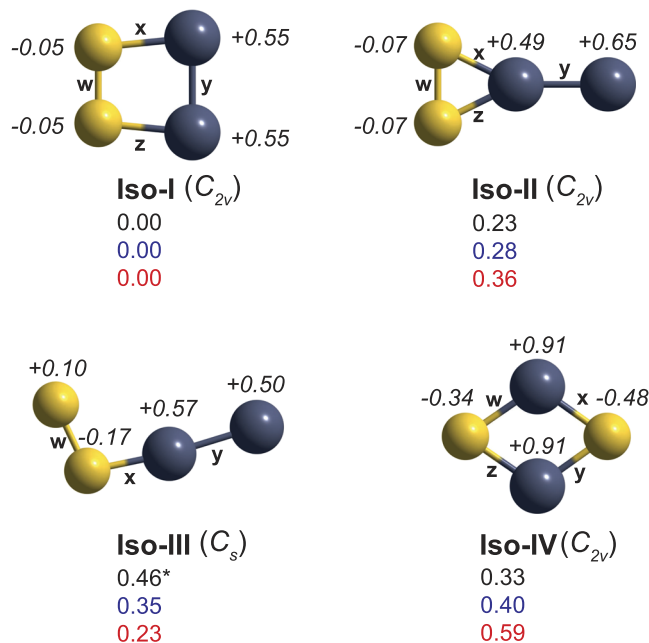
FIG. 3. Lowest lying \text{Cd}_2\text{Se}_2^+ isomers (Cd: dark atoms, Se: light atoms) and their relative energies in eV, as obtained at the CCSD(T)/cc-pVTZ (black), PBE0/cc-pVTZ-PP (blue), and B3LYP/cc-pVTZ-PP (red) levels of theory together with their point group symmetries. The star * indicates the CCSD(T) energy calculation for the geometry relaxed at the PBE0/cc-pVTZ-PP level of theory. Natural charges from NBA are given in italic font. The chemical bonds are labeled with w, x, y, and z.
