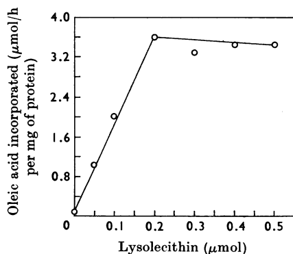
Fig. 2. Effect of lysolecithin concentration on the acyl-transferase activity of brush-border-free mucosa. Incubations were carried out for 10 min at 37^\circ\text{C} .
