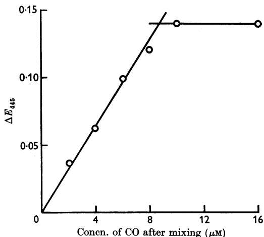
Fig. 4. Titration of reduced cytochrome oxidase (Yonetani preparation) with CO. The enzyme [20.5 \mu M (expressed as haem) after mixing] was allowed to react at 24° in the stopped-flow apparatus with various concentrations of CO dissolved in 0.1 M-phosphate buffer, pH 7.4. The reaction was followed at 445 m \mu in a 2 mm. light-path and the total change in extinction is plotted against the concentration of CO.
