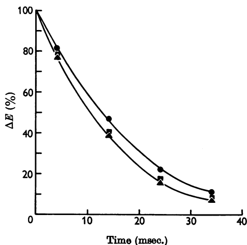
Fig. 9. Reaction of 2 \mu M-O_2 with an approximately equivalent amount of reduced cytochrome oxidase (Greenwood preparation) followed at 605 m\mu (▲), 445 m\mu (●) and 410 m\mu (■). The enzyme was dissolved in tris-HCl buffer, pH 8.5. Other conditions were: temperature, 21^\circ ; light-path, 2 cm. The results are expressed as percentages of the total change in extinction between the first observation 4 msec. after mixing and 100 msec. after mixing.
