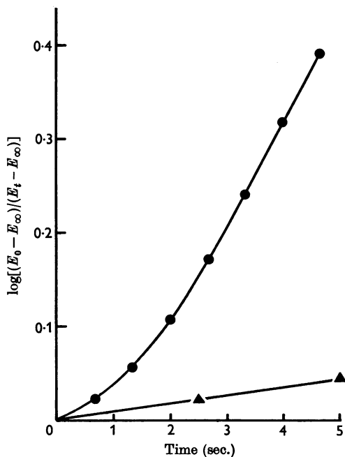
Fig. 3. Displacement of CO from reduced cytochrome oxidase (Yonetani preparation) by NO (▲), and the oxidation of the CO compound of reduced cytochrome oxidase by O_2 (●). The CO compound of reduced cytochrome oxidase [ 4 \mu\text{M} (expressed as haem) after mixing] was mixed in the stopped-flow apparatus with 300 \mu\text{M} NO and the reaction followed with light of mean wavelength 430 \text{ m}\mu at 21^\circ in 0.1 \text{ M} -phosphate buffer, pH 7.4; a 2 cm. light-path was used. In the oxidation experiment the same enzyme solution was mixed with air-equilibrated phosphate buffer to give a concentration of O_2 after mixing of 140 \mu\text{M} . The reaction was followed with light of mean wavelength 445 \text{ m}\mu . The Figure shows \log[(E_0 - E_\infty)/(E_t - E_\infty)] plotted against time in each case. The first-order rate constant for the replacement of CO by NO was 0.023 \text{ sec}^{-1} .
