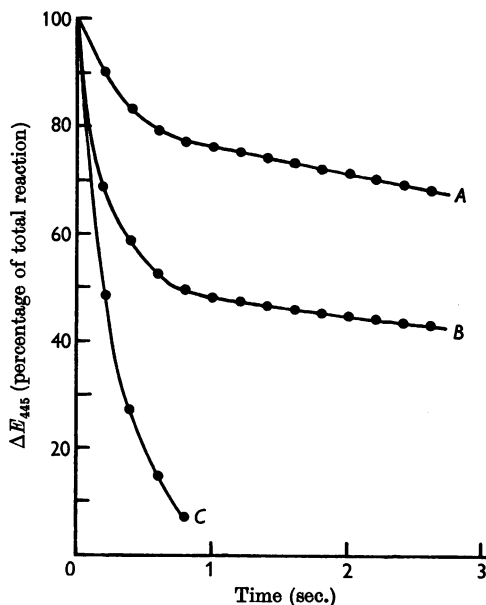
Fig. 15. Changes in extinction at 445 \text{ m}\mu when reduced enzyme (Yonetani preparation) [ 2.5 \mu\text{M} (expressed as haem) after mixing] was allowed to react with 50 \mu\text{M} -CO. The enzyme solution contained: A, 1.5 \text{ mM} -KCN; B, 0.44 \text{ mM} -KCN; C, no cyanide. Other conditions were: temperature, 23°; 0.1 \text{ M} -phosphate buffer, pH 7.4.
