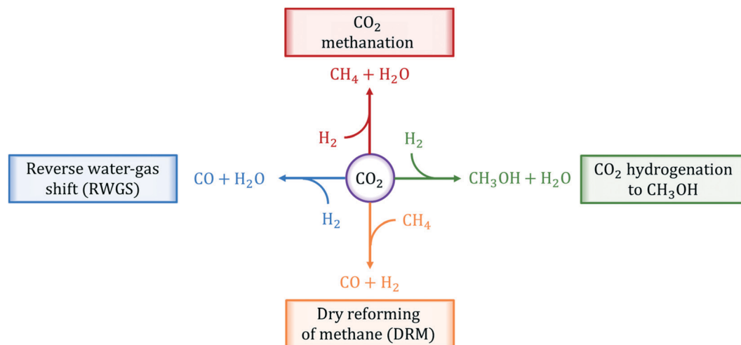
Fig. 1 Chemical reactions of thermo-catalytic activation and conversion of CO 2 to C 1 products reviewed in this work.
