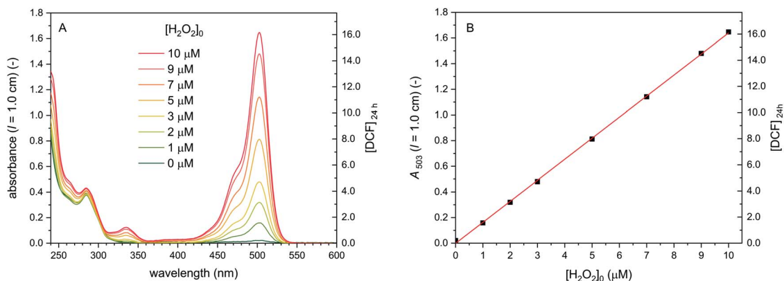
Fig. 8 Cascade reactions 5 (in bulk solution) with [DCFH_2-DA]_0 = 50 \mu M , [BCA] = 1.0 \mu M , [HRP] = 10 nM, and [H_2O_2]_0 = 0 – 10 \mu M , PB (pH = 7.2), 1 vol% DMSO, T = 25^\circ C . (A) UV/vis spectrum of the reaction mixtures measured after t = 24 h. (B) A_{503} ( t = 24 h) vs. [H_2O_2]_0 . The concentration of DCF obtained after t = 24 h is shown on the right hand side. Spectral fitting showed that DCF_{ox} did not form. Linear regression for the data points for [H_2O_2]_0 = 0 – 10 \mu M is shown (coefficient of determination, R^2 = 0.99969 ).
