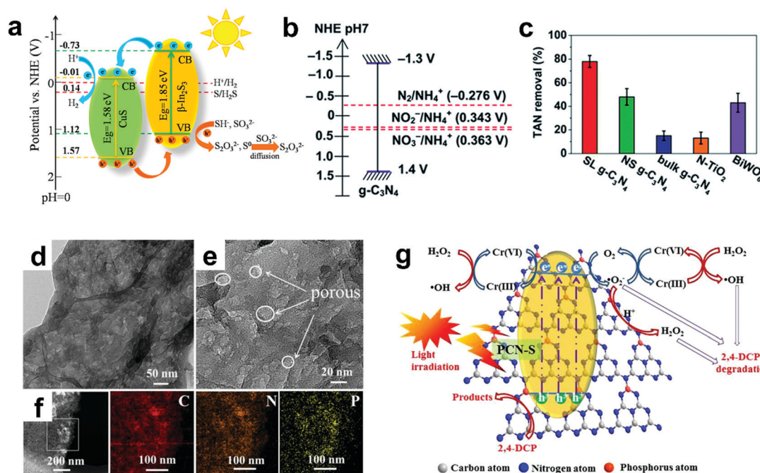
Fig. 19 Photocatalysts based on 2D nanomaterials for the removal of inorganic pollutants. (a) Photocatalytic degradation of H 2 S by In 2 S 3 /CuS composites under visible light irradiation. Reproduced with permission. 333 Copyright 2018, Elsevier B.V. (b) Illustration of the band structure of g-C 3 N 4 with redox levels for ammonia oxidation. (c) Comparison of the photocatalytic performance of samples of single-layer g-C 3 N 4 (SL g-C 3 N 4 ), g-C 3 N 4 nanosheets (NS g-C 3 N 4 ), bulk g-C 3 N 4 , N-doped TiO 2 (N-TiO 2 ), and Bi 2 WO 6 for pollutant removal under Xe lamp irradiation. (b and c) Reproduced with permission. 334 Copyright 2014, the American Chemical Society. (d) Low- and (e) high-resolution of TEM images of P-doped C 3 N 4 nanosheets (PCN-S), and (f) STEM of PCN-S and corresponding elemental mapping. (g) Schematic illustration of the simultaneous removal of Cr(VI) and 2,4-DCP using PCN-S photocatalyst. (d–g) Reproduced with permission. 336 Copyright 2017, Elsevier B.V.
