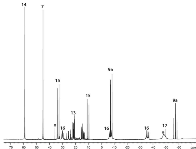
Fig. 8 ^{31}\text{P} NMR spectrum of the reaction of 7 with \text{Cy}_2\text{PH} in a 1 : 1 ratio in \text{CD}_2\text{Cl}_2 after 3.5 h; unidentified products are marked with asterisks.
