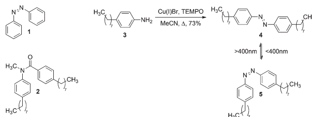
Scheme 1 Azobenzene ( 1 ), a lipid-interactive benzanilide ( 2 ) and the conformationally similar azobenzene derivatives studied here ( 4 and 5 ), and their synthesis.
