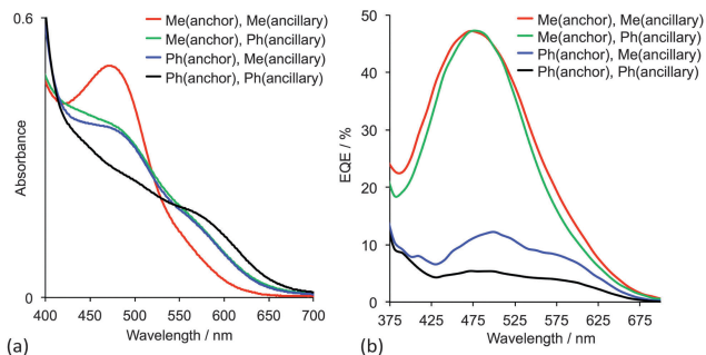
Fig. 9 (a) Solid-state absorption spectra and (b) EQE spectra of \text{TiO}_2 electrodes with adsorbed dyes containing 6,6'- \text{Me}_2\text{bpy} or 6,6'- \text{Ph}_2\text{bpy} copper-binding domains. 30 The ligands are shown in Fig. 8b.
