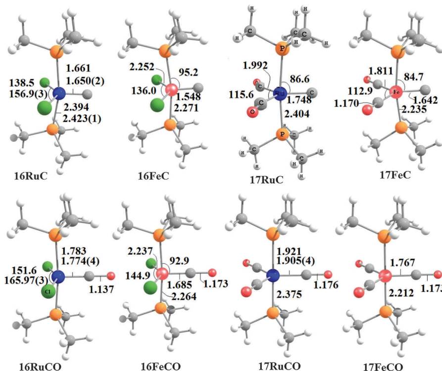
Fig. 17 Calculated geometries (BP86/TZ2P) of the carbon complexes 16TMC and 17TMC and the carbonyl complexes 16TMC O and 17TMC O. Bond lengths are given in Å, angles in degree. 75 Experimental data are given in italics . 2,76a,b The figure has been adapted from ref. 75.
