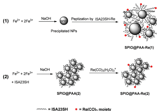
Scheme 1 The synthetic routes used in this work for preparing the SPIO@PAA nanomaterials, containing iron oxide nanocrystals coated with the poly(amido)-amine (PAA) ISA23SH, decorated with \text{Re(CO)}_3 units.
