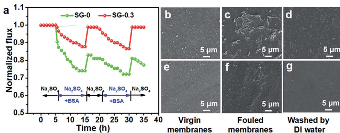
Fig. 7 (a) Time-dependent relative water flux of SG-0 and SG-0.3 membrane tested with 2\text{ g L}^{-1}\text{ Na}_2\text{SO}_4 and 2\text{ g L}^{-1}\text{ Na}_2\text{SO}_4 + 1\text{ g L}^{-1}\text{ BSA} aqueous solution at 25^\circ\text{C} and 6 bar; SEM images of SG-0 (b–d) and SG-0.3 (e–g) surface after antifouling experiment.
