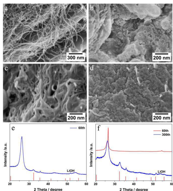
Fig.8 SEM micrographs of MWNTs cathode prior to use (a), MWNTs cathode after 60 cycles in the cell with GF separator (b), MWNTs cathode after 60 (c) and 300 cycles (d) in the cell with the PU/SiO 2 /GF separator, as well as the XRD patterns of the MWNTs cathode in the cells with the GF separator after 60 cycles (e) and with the PU/SiO 2 /GF separator after 60 and 300 cycles (f), respectively. Electrolyte: 0.05 M LiI and 1 M LiClO 4 dissolved in DMSO.
