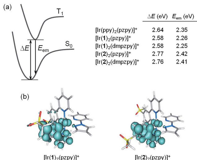
Fig. 8 (a) Schematic diagram showing the adiabatic energy difference (ΔE) between S 0 and T 1 and the emission energy (E em ) from T 1 computed for [Ir(ppy) 2 (pzpy)] + and for complexes [Ir(C ^ N) 2 (N ^ N)] + (C ^ N = [1] - and [2] - , N ^ N = pzpy and dmpzpy). (b) Unpaired-electron spin density contours (0.002 au) calculated for the fully relaxed T 1 state of [Ir(1) 2 (pzpy)] + and [Ir(2) 2 (pzpy)] + .
