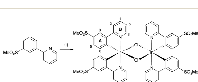
Scheme 5 Synthetic route to [Ir(2) 2 Cl] 2 . Conditions: (i) [Ir(cod)Cl] 2 , 2-ethoxyethanol, N 2 , overnight, reflux. Numbering scheme is for NMR spectroscopic assignments.
