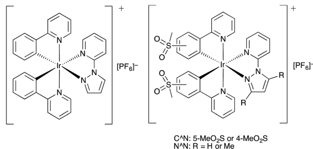
Scheme 3 Structures of [Ir(ppy) 2 (pzpy)][PF 6 ] 8 and methylsulfonyl-substituted complexes [Ir(C ^ N) 2 (N ^ N)][PF 6 ] + with C ^ N = [1] – or [2] – , and N ^ N = 2-(1 H -pyrazol-1-yl)pyridine (pzpy) or 2-(3,5-dimethyl-1 H -pyrazol-1-yl)pyridine (dmpzpy).
