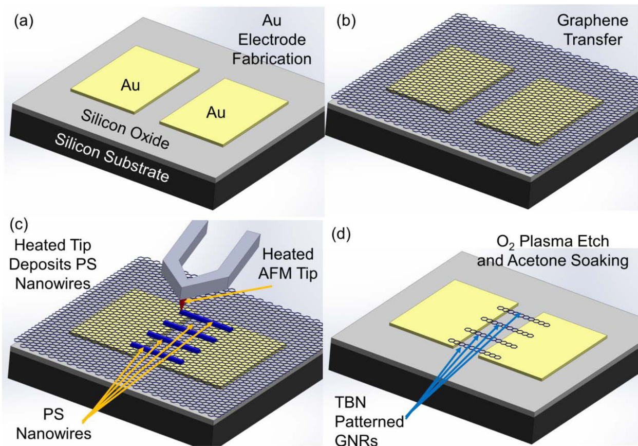
Figure 1. Schematics illustrating major steps of GNR fabrication using TBN method with a heated AFM tip.
