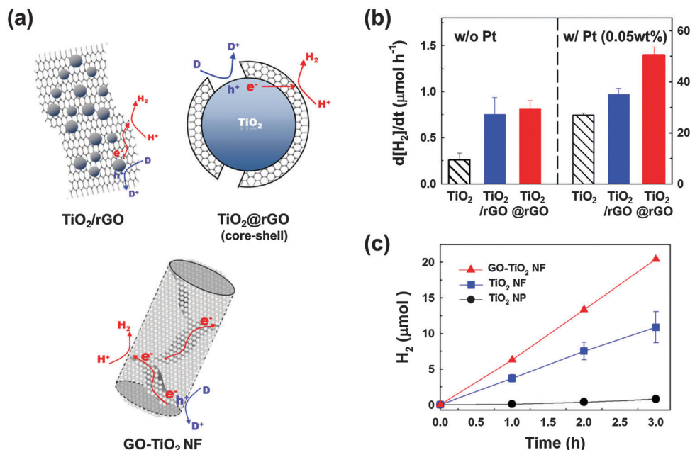
Fig. 6 (a) Illustration of the various composite structures of TiO 2 and (r)GO sheets and the associated charge transfers for hydrogen production. (b) Photocatalytic H 2 production rates in the aqueous suspensions of TiO 2 , TiO 2 dispersed on a 2D rGO sheet, and the TiO 2 /rGO core/shell structure before (left panel) and after Pt loading (right panel). (c) Time profiles of H 2 production in the aqueous suspensions of TiO 2 nanoparticles (NPs), TiO 2 nanofibers (NFs), and GO embedded in TiO 2 NFs (GO–TiO 2 NF). (a and b) Adapted with permission from ref. 149 (Copyright 2012 American Chemical Society). (a and c) Reprinted from ref. 152 with permission by Elsevier.
