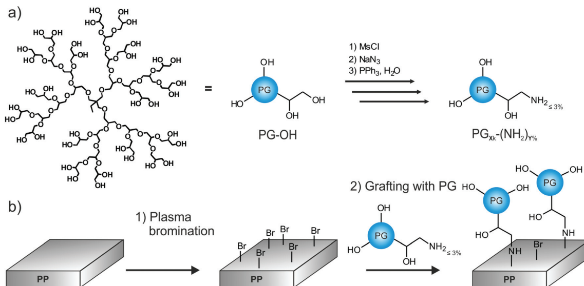
Fig. 1 (a) Synthesis of polyglycerols (PG) \text{PG}_{\text{Xk}}\text{-(NH}_2\text{)}_{y\%} with different molecular weights and amounts of amino functionalization. An idealized structure of PG is shown. (b) Schematic representation of the two-step synthesis of PG-lated polypropylene (PP) surfaces by (1) plasma bromination and (2) grafting with PG.
