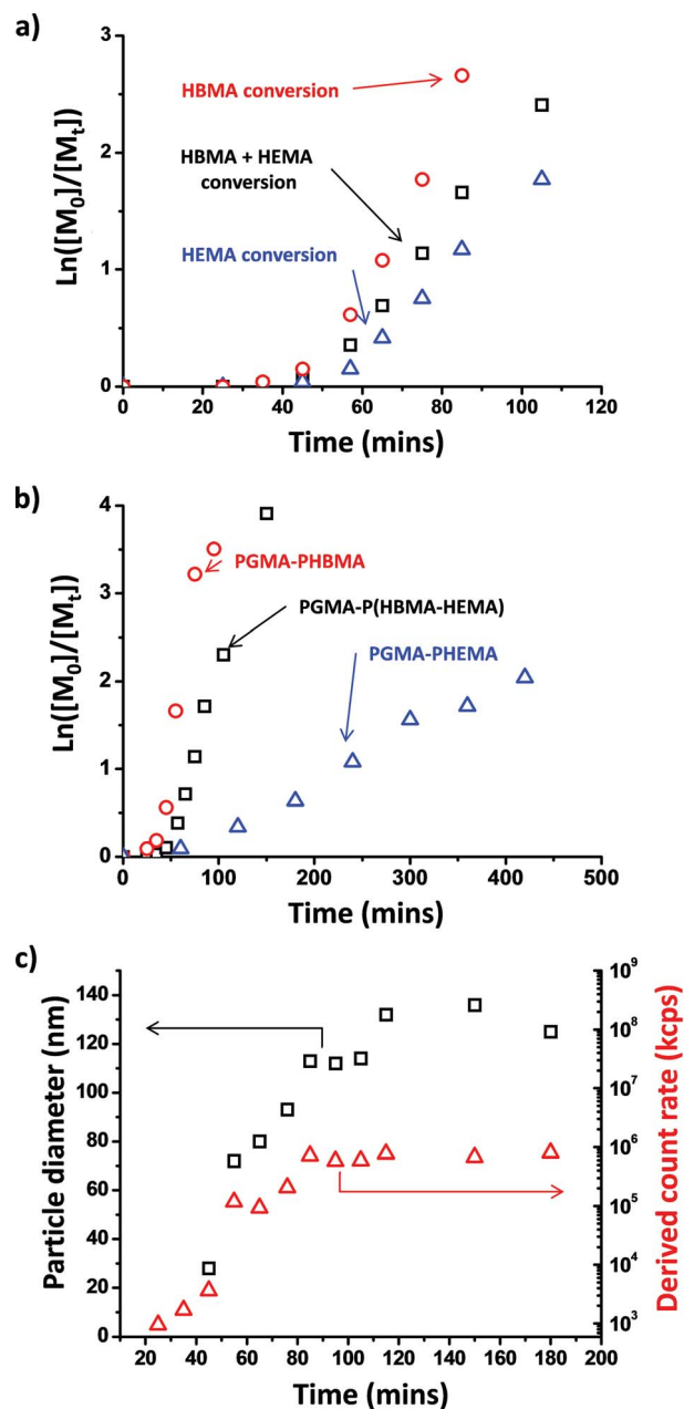
Fig. 6 Semi-logarithmic plot of monomer conversion vs. time determined by ^1\text{H} NMR analysis of periodically-sampled aqueous reaction mixtures at 70 °C using a macro-CTA/ACVA molar ratio of 4.0 for: (a) overall rate for the RAFT statistical copolymerization of a 1 : 1 HBMA/HEMA molar ratio when targeting \text{PGMA}_{60}\text{-P}(\text{HBMA}_{268}\text{-HEMA}_{268}) at 10% w/w solids (black squares), and the corresponding individual rates of polymerization of HBMA (red circles) and HEMA (blue triangles) determined for the same copolymerization. (b) Overall rate of RAFT statistical copolymerization for the same \text{PGMA}_{60}\text{-P}(\text{HBMA}_{268}\text{-HEMA}_{268}) formulation compared to the overall rates for the RAFT emulsion homopolymerization of HBMA (targeting \text{PGMA}_{60}\text{-PHBMA}_{536} at 10.8% w/w solids) and RAFT solution homopolymerization of HEMA (targeting \text{PGMA}_{60}\text{-PHEMA}_{536} at 9.2% w/w total solids). (c) Evolution of intensity-average particle diameter (black squares) and count rate (kcps, red triangles) over time for a periodically-sampled \text{PGMA}_{60}\text{-P}(\text{HBMA}_{268}\text{-HEMA}_{268}) statistical copolymerization prepared at 10% w/w solids, as determined by DLS studies. The onset of micellar nucleation was observed at approximately 45 min, and was accompanied by a pronounced increase in the scattered light intensity.
