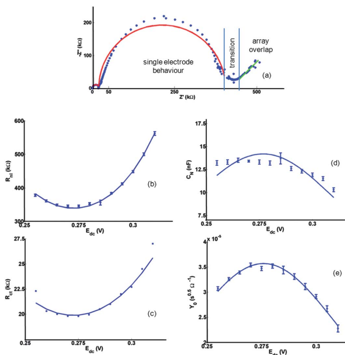
Fig. 7 (a) Typical subtracted Nyquist Electrochemical Impedance Spectroscopy (EIS) data at the 10\mu\text{SD50n} electrode for oxidation of FCA(I) solution at E_{\text{dc}} = +0.290 V. Also shown are theoretical fits to the circuit in Fig. 4c and to the circuit (resistance in series with Warburg element) appropriate at low frequency when there is complete diffusional array overlap. Fits (solid lines) to the (b) R_{\text{nl}} (c) R_{\text{ct}} (d) C_{\text{N}} (e) Y_0 data extracted from iterative fitting to the EIS measurements at each E_{\text{dc}} performed using either Matlab (The Mathworks, Natick, Massachusetts, USA) or Nova (Version 1.9, Metrohm Autolab B.V., Utrecht, The Netherlands). The fits of these data to eqn (3), (8), (10) and (13), (lines shown in (b), (c), (d) and (e)) gave the following global values: E' = 0.273 \pm 0.002 V; R_{\text{ct}}^{\text{min}} = 19.87 \pm 0.06 k \Omega ; R_{\text{nl}}^{\text{min}} = 339 \pm 1 k \Omega ; C_{\text{N}}^{\text{max}} = 14.3 \pm 0.3 nF; Y_0^{\text{max}} = 35.7 \pm 0.2 \mu\text{s}^{0.5} \Omega^{-1} .
