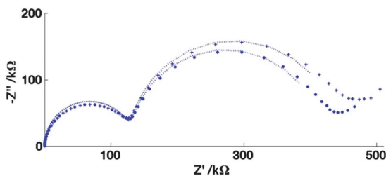
Fig. 11 EIS data for the 20\mu\text{m} 3D50n electrode showing the oxidation of 0.1 mM FCA in FCA(I) solution (+) and FCA(//10) solution (●) and the corresponding fits for E_{dc} = E' , V_{ac} = 10 \text{ mV} , for the frequency range 100 kHz to 10 mHz (logarithmic distribution). Fits: FCA(I) solution: R_{ct} = 135 \pm 1 \text{ k}\Omega , C_{dl} = 31.1 \pm 0.7 \text{ nF} , R_{nl}^{\text{min}} = 309 \pm 3 \text{ k}\Omega , C_N = 1.34 \pm 0.02 \mu\text{F} , FCA(//10) solution: R_{ct} = 135 \pm 1 \text{ k}\Omega , C_{dl} = 27.7 \pm 0.6 \text{ nF} , R_{nl}^{\text{min}} = 283 \pm 2 \text{ k}\Omega , C_N = 1.33 \pm 0.02 \mu\text{F} .
