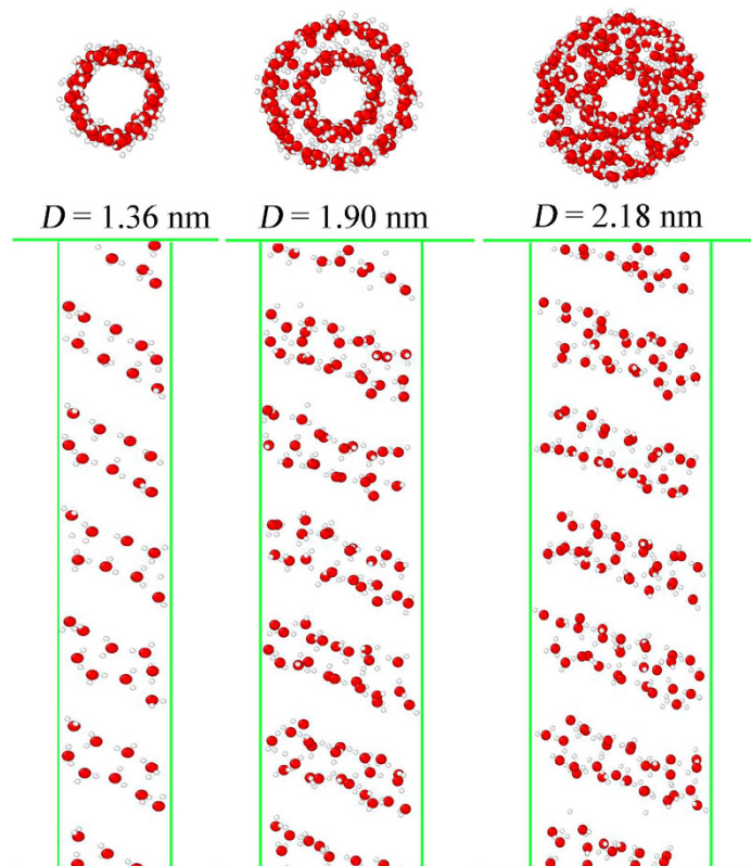
Figure 7. (Top panel) Top view of water structures inside the screw pumps with D = 1.36 , 1.90 and 2.18 nm. (Bottom panel) Corresponding water structures inside the back half tube from side view. Green lines denote outlines for CNT and graphene.
