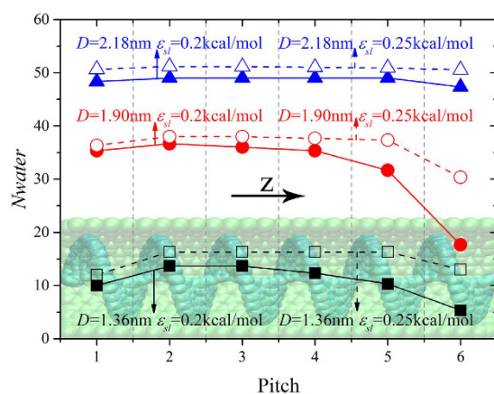
Figure 8. Number of water molecules in each screw pitch ( N_{water} ) along the z direction. For D = 1.36 , 1.90 and 2.18 nm, the results are shown by square, circle and triangle. For each screw's diameter, results are provided when \epsilon_{ls} = 0.2 kcal/mol and \epsilon_{ls} = 0.25 kcal/mol, which are denoted by solid and hollow symbols, respectively. The points are connected to guide the eye. The inset shows the schematic of corresponding pitch along the z direction.
