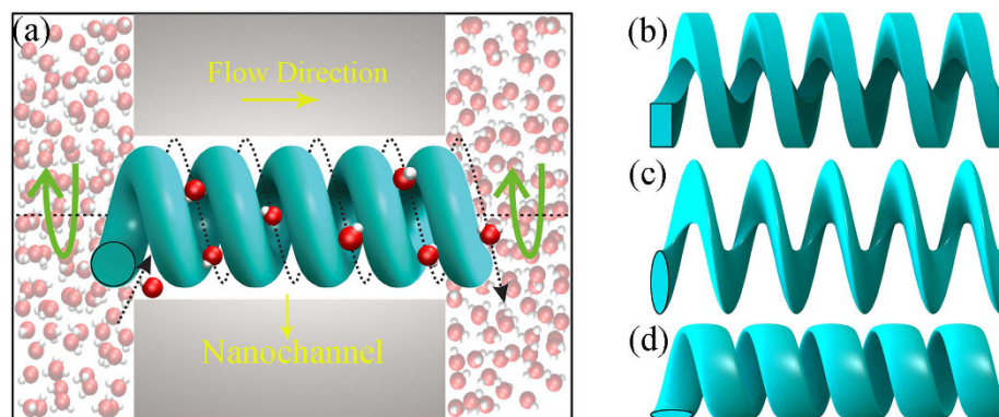
Figure 1. Design concept of the nano screw pump. (a) By virtue of the rotating helical nanowire with circular cross section embedded inside a nanochannel, water molecules are transported directed in a helical fashion. The trajectory of a single water molecule is illustrated by the dotted line. (b) Helical nanowires with rectangular cross section. (c) Normal helical nanowire. (d) Binormal helical nanowire.
