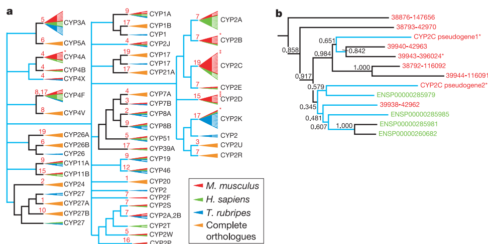
Figure 20 Cytochrome P450 protein families in mouse, human and pufferfish. a , Phylogenetic tree, based on the neighbour-joining method 297 , applied to the alignment of the whole P450 protein family. Each triangle represents a cytochrome P450 family cluster. Asterisks next to a triangle represent mouse pseudogenes defined by the presence of either an in-frame stop codon or a frameshift. The colour codes are indicated in the lower-right panel. When the family presents one member in each of the studied organisms, the triangle is labelled in orange. The height of the triangle is proportional to the number of proteins, which is indicated by white-line subdivisions. Chromosomal location in mouse is shown on each of the branches for each subfamily. The lengths of the branches are not drawn to scale. Branches with significant nodes (bootstrapping value >0.7) are in black, with the remainder in blue. In 6 out of the 15 CYP2C family cases, the
