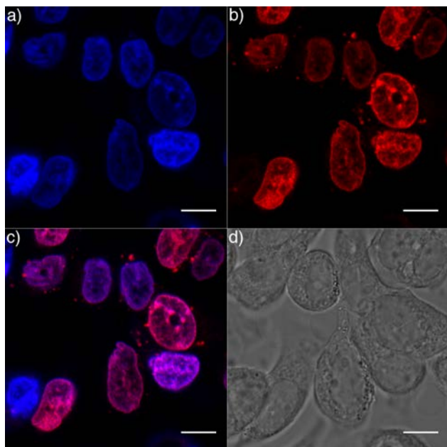
Figure 6. Free DOX accumulates in the nucleus of LIM1899 cells as visualized by CSLM (c, overlay). Cells were treated with DOX (1 \mu M) in growth media at 37 °C, 5%CO 2 for 24 h. The nuclei were counterstained with Hoechst 33342 (a, blue) and the intracellular distribution of DOX was visualized by confocal microscopy (b, red). Brightfield image of the cells is shown in gray (d). Scale bars, 10 \mu m.
