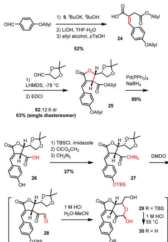
Scheme 2. Revised Synthesis of Plagiogyrin A Core
