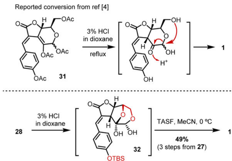
Figure 5. Acid-promoted hemiacetal formation.
