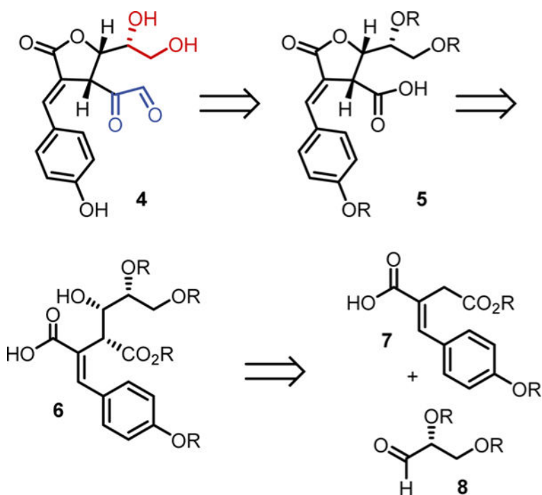
Figure 3. Retrosynthetic approach to diol 4 .
