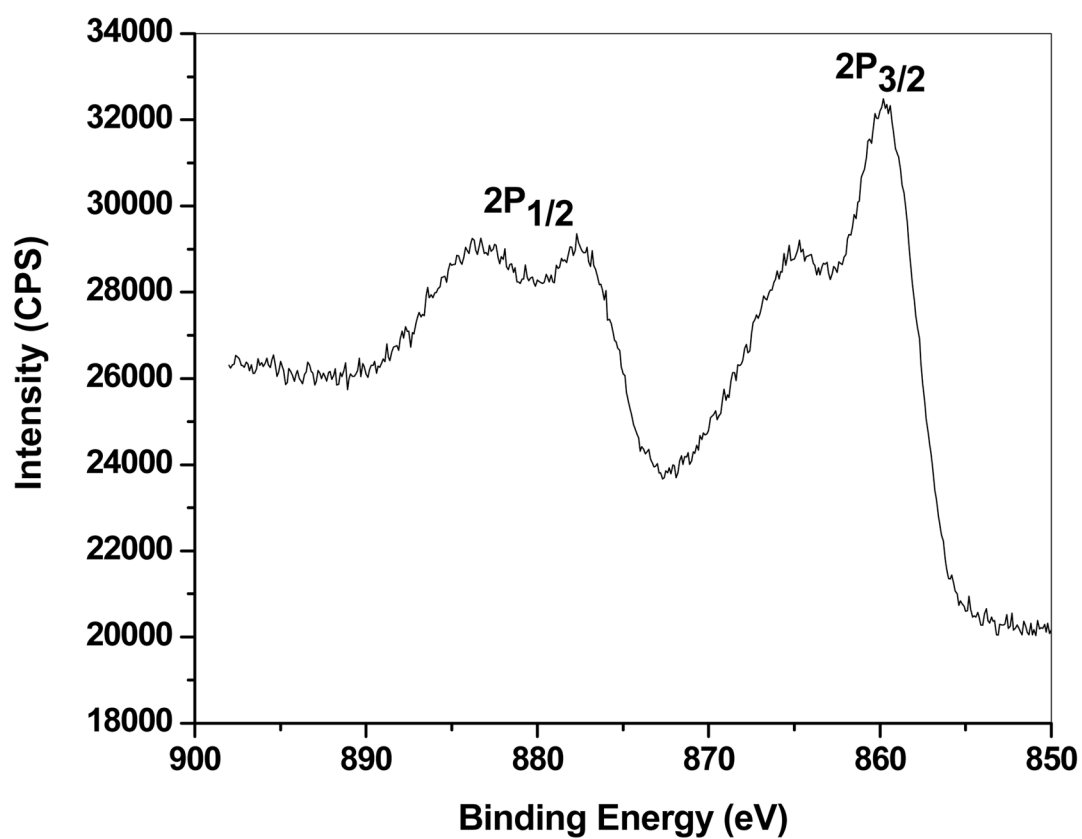
Figure 1. X-ray photoelectron spectroscopic (XPS) data of \text{SiO}_2\text{-TMR-NTA-Ni}^{2+} ( 1 ), showing the Ni ion peak section.
