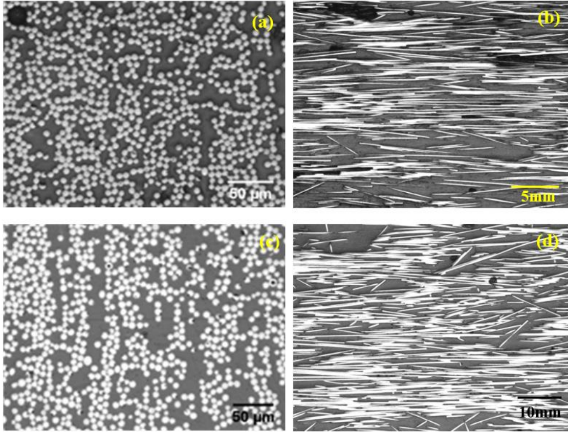
Figure 6 Micrograph of aligned composite cross section and in-plane view: (a)(b)3mm_46% fibre volume fraction; (c)(d)12mm_43% fibre volume fraction
