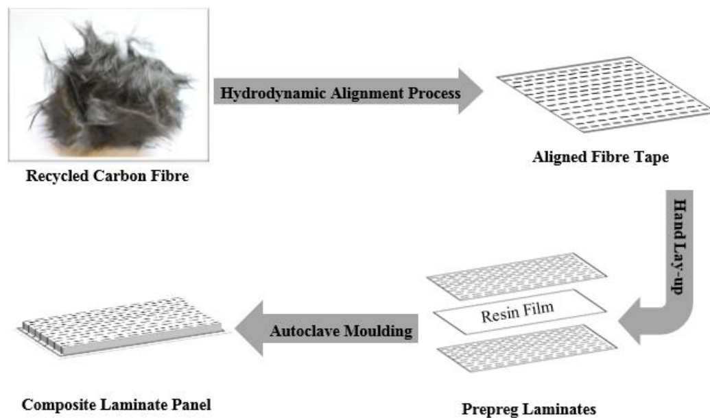
Figure 2 A schematic representation of the manufacturing process of aligned fibre laminate composites
