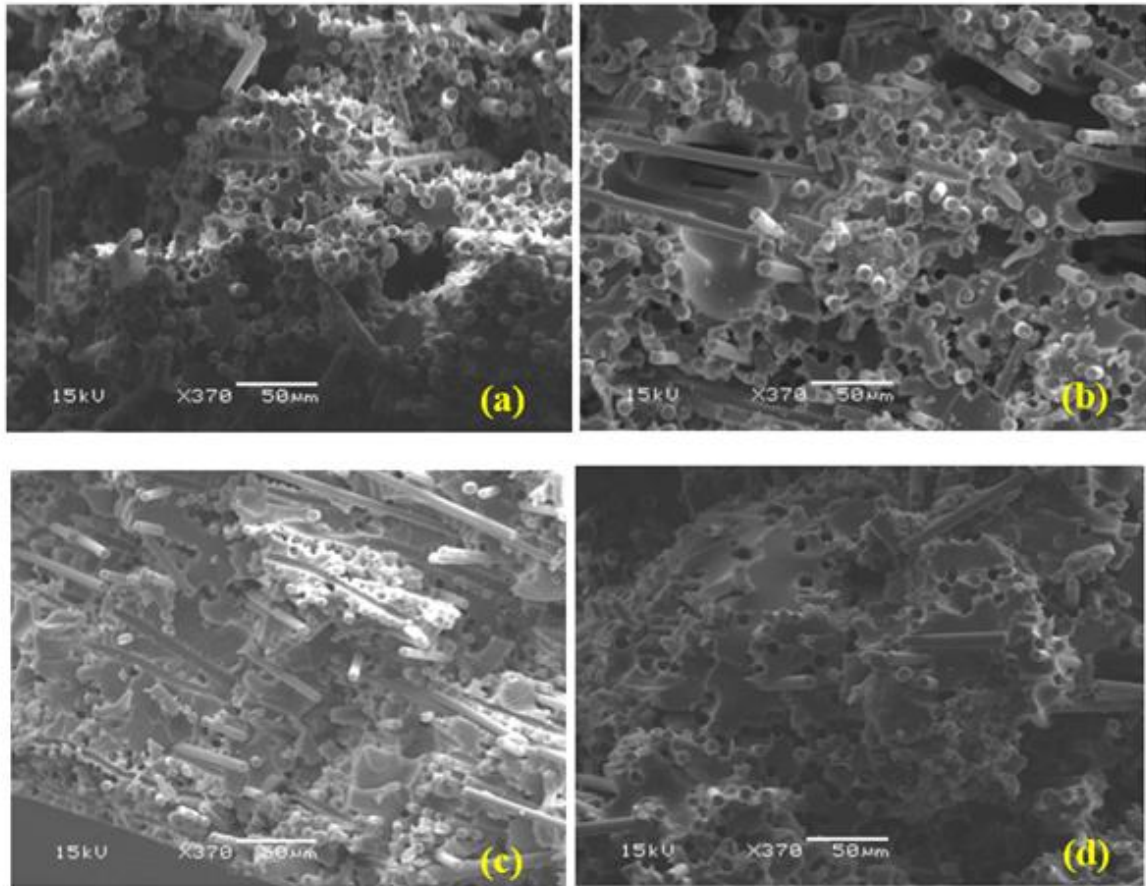
Figure 8 Fracture surface images obtained by SEM: (a) 3mm fibre specimen; (b) 12mm fibre specimen; (c) recycled fibre specimen; (d) 7mm_T800 fibre specimen
