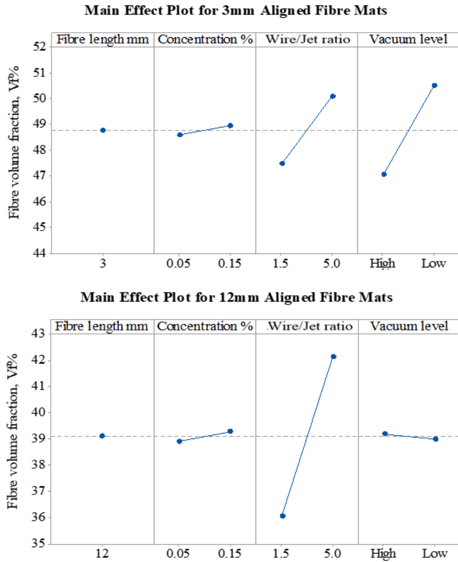
Figure 4 Main effect plots of compaction test results from full factorial DoE
