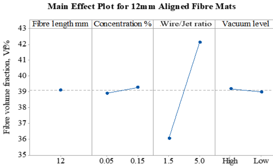
Figure 4 Main effect plots of compaction test results from full factorial DoE
