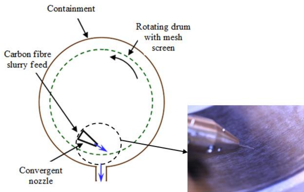
Figure 1 A schematic representation of the hydrodynamic alignment process
