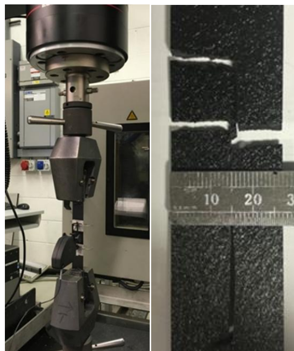
Figure 3 Tensile testing setup and typical fracture cross section of 3mm fibre laminate composite specimen
