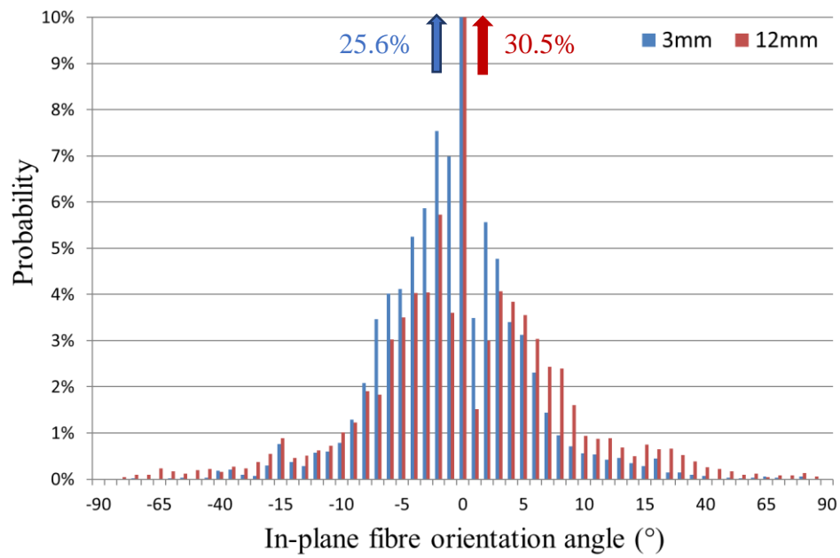
Figure 7 In plane fibre orientation distribution for composite specimens made by 3mm fibre (fibre orientation distribution factor \eta_0 = 0.977 ) and 12mm fibre (fibre orientation distribution factor \eta_0 = 0.949 ). Note that the y-axis is truncated.
