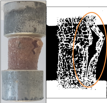
c) Splitting fracture
