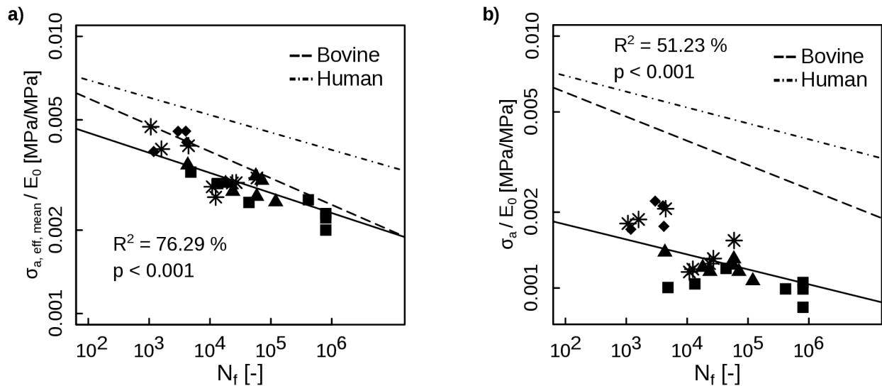
Figure S2: Fatigue life curve for the normalized stress amplitude with respect to the initial elastic modulus. The stress amplitudes were calculated based on the mean effective area (a) and the nominal area of the trabecular specimens (b). The results were compared with fatigue life of human vertebrae [1].and bovine trabecular [2].
