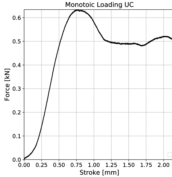
Figure S1: A typical force-displacement curve for trabecular specimens tested under monotonic compression loading.
