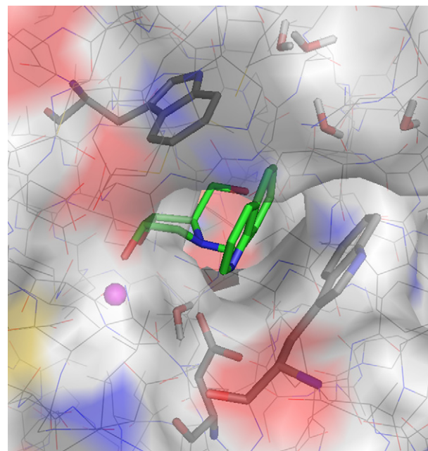
Figure 4. Binding of inhibitor 42 in the active site of the target enzyme. The nucleobase mimic is orientated parallel between Trp83 and Trp260, enabling aromatic stacking interactions. The active site residues are depicted in grey (carbons), blue (nitrogens), and red (oxygen). The carbons of the inhibitor are depicted in green, the color codes for nitrogens and oxygens are the same as for the active site residues. Water molecules are depicted as red spheres, the Ca^{2+} ion is depicted as a magenta sphere. The colors of the enzyme surface are according to the elements. The image was made with PyMOL (PyMOL Molecular Graphics System, DeLano Scientific, San Carlos, CA).
