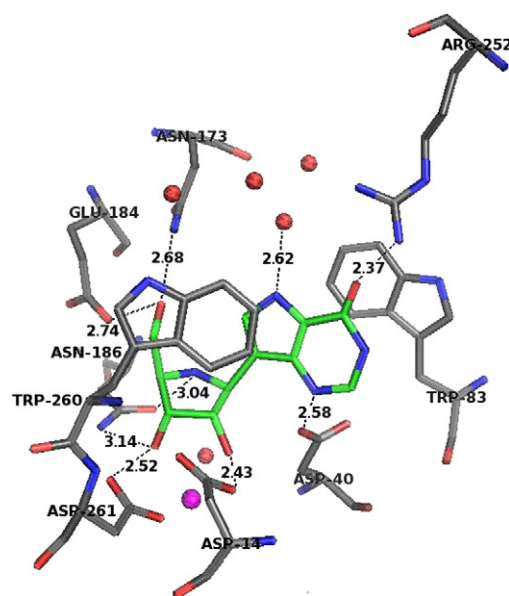
Figure 1. The active site of Tv NH co-crystallized with Immucillin-H (pdb code 2FF2). 11 Interaction distances are given in Å. The active site residues are depicted in grey (carbons), blue (nitrogens), and red (oxygens). The carbons of the inhibitor are depicted in green, the color codes for nitrogens and oxygens are the same as for the active site residues. Water molecules are depicted as red spheres, the \text{Ca}^{2+} ion is depicted as a magenta sphere. The image was made with PyMOL (PyMOL Molecular Graphics System, DeLano Scientific, San Carlos, CA).
