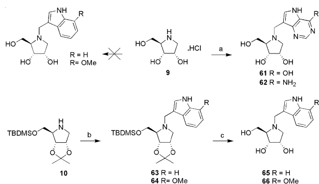
Scheme 3. Reagents and conditions: (a) 9-deazahypoxanthine or Boc-protected 9-deaza-adenine, aq \text{CH}_2\text{O} , NaOAc, \text{H}_2\text{O} , 95^\circ\text{C} , 17 h; (b) indole or 7-methoxy-indole, aq \text{CH}_2\text{O} , \text{H}_2\text{O} /dioxane 1:1, 95^\circ\text{C} , 20 h; (c) TFA/ \text{H}_2\text{O} 1:1, rt, 18 h.
