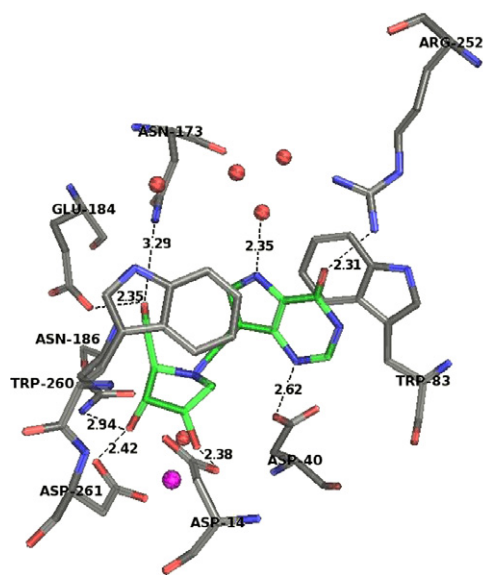
Figure 2. Inhibitor 61 in the active site of the target enzyme. Interaction distances are given in Å. Color codes are the same as for Figure 1. The images were made with PyMOL (PyMOL Molecular Graphics System, DeLano Scientific, San Carlos, CA).
