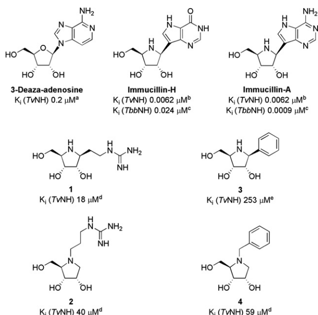
Chart 1. Inhibitors against purine specific NH (TvNH = IAG-NH from T. vivax ; TbbNH = IAG-NH from T. brucei brucei ). Data taken from a J. Mol. Biol. 2001 , 307, 1363–1379, b J. Mol. Biol. 2006 , 359, 331–346, c Biochemistry 1999 , 38, 13147–13154, d Eur. J. Med. Chem. 2008 , 43, 315–326, e unpublished results from our group.
