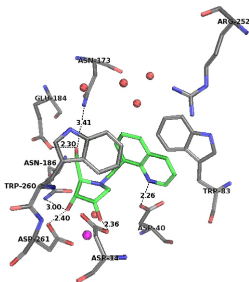
Figure 3. Inhibitor 42 in the active site of the target enzyme. Interaction distances are given in Å. Color codes are the same as for Figure 1. The images were made with PyMOL (PyMOL Molecular Graphics System, DeLano Scientific, San Carlos, CA).
