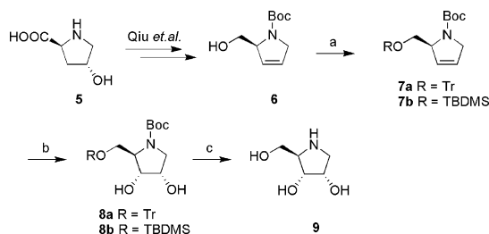
Scheme 1. Reagents and conditions: (a) TrCl, pyridine, rt, 24 h, or TBDMSCl, imidazol, Et 3 N, CH 2 Cl 2 , rt, 18 h; (b) K 2 OsO 4 ·2H 2 O, 4-methylmorpholine N -oxide, acetone, H 2 O, rt, 18 h; (c) TFA/H 2 O 1:1, rt, 18 h.
