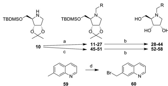
Scheme 2. Reagents and conditions: (a) Procedure A: arylmethylhalide, \text{Na}_2\text{CO}_3 , \text{CH}_2\text{Cl}_2 , \text{H}_2\text{O} , reflux, 3–20 h, Procedure B: arylmethylhalide, \text{K}_2\text{CO}_3 or \text{KHCO}_3 , DMF, 40^\circ\text{C} , 1.5–4 h; (b) TFA/ \text{H}_2\text{O} 1:1, rt, 18 h; (c) Procedure for the synthesis of 52 : 4-pyridinecarboxaldehyde, \text{NaCNBH}_3 , MeOH, rt, 24 h; Procedure for the synthesis of target compounds 53–58 : arylcarboxaldehyde, \text{CH}_2\text{Cl}_2/\text{AcOH} 10/1, (polystyrylmethyl)trimethylammonium cyanoborohydride, rt, 28 h; (d) N -bromosuccinimide, dibenzoylperoxide, \text{CCl}_4 , reflux, 18 h.
