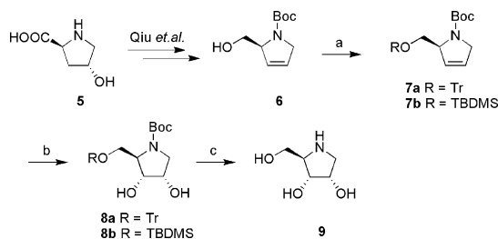
Scheme 1. Reagents and conditions: (a) TrCl, pyridine, rt, 24 h, or TBDMSCl, imidazole, Et 3 N, CH 2 Cl 2 , rt, 18 h; (b) K 2 OsO 4 ·2H 2 O, 4-methylmorpholine N -oxide, acetone, H 2 O, rt, 18 h; (c) TFA/H 2 O 1:1, rt, 18 h.
