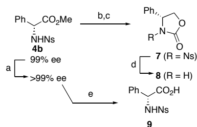
Scheme 1. Reagents and conditions: (a) recrystallization from EtOH, 91%. (b) DIBAL-H, \text{CH}_2\text{Cl}_2 , -78\text{ }^\circ\text{C} to 0\text{ }^\circ\text{C} , 0.5 h; (c) triphosgene, \text{Et}_3\text{N} , \text{CH}_2\text{Cl}_2 , 0\text{ }^\circ\text{C} , 1 h, 88% (2 steps); (d) \text{PhSH} , \text{Cs}_2\text{CO}_3 , DMF, 23\text{ }^\circ\text{C} , 1 h, 81%; (e) LiI, EtOAc, reflux, 6 h, 94%
