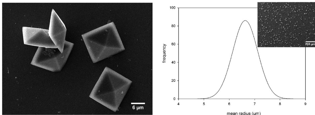
Fig. 1. Size distribution of the weddellite crystals obtained from the experiment G4.
