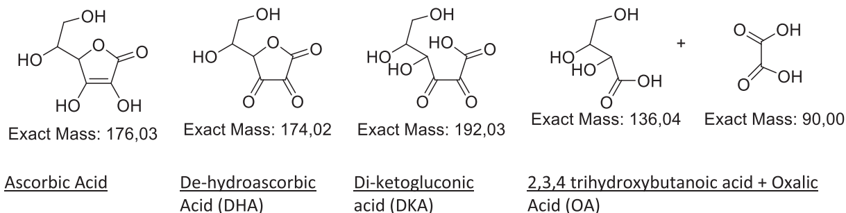
Scheme 1. Degradation products starting from Ascorbic acid at pH = 2.
