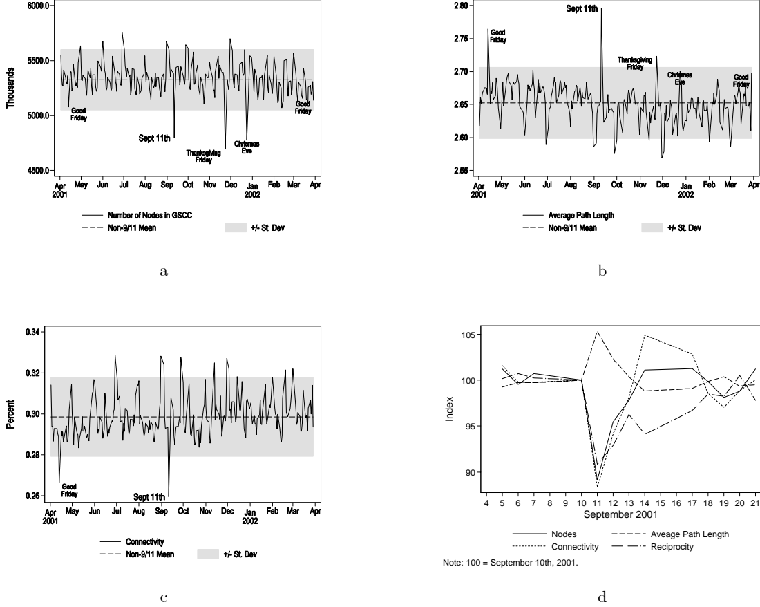
FIG. 5: a) Number of nodes, n , in giant strongly connected component (GSCC) April 2001 - April 2002. b) Average path length, \langle \ell \rangle , April 2001 - April 2002 c) Connectivity, p , in GSCC, April 2001 - April 2002 d) Size, average path length, connectivity and reciprocity Sept. 4 - 21, 2001, Sept. 10, 2001 = 100
