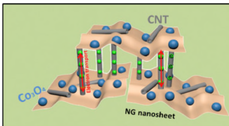
Figure 39. Schematic representation of structure and energy storage characteristics of the \text{Co}_3\text{O}_4/\text{NG}/\text{CNTs} composite. Reprinted with permission [121]. Copyright 2015 Elsevier.
