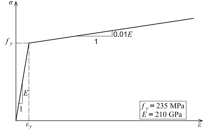
Figure 4: Bi-linear material curve with a yield stress of f_y = 235 MPa and a hardening slope of E/100 as used for the primary investigations of this paper.
