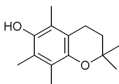
4: 2,2,5,7,8-Pentamethyl-6-chromanol
