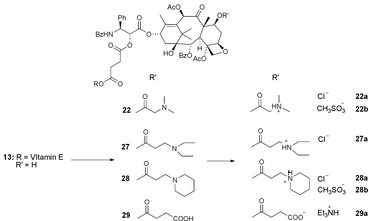
Scheme 2.
