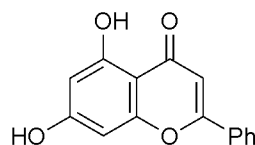
9: Chrysin
