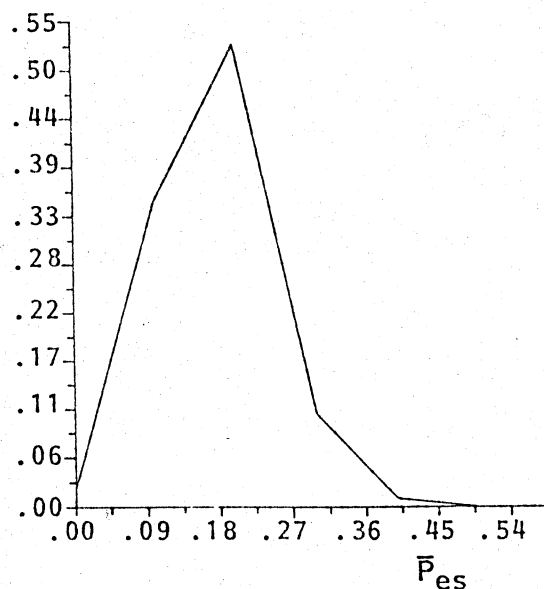
Fig. 4: Marginal density function of \bar{P}_{es}
