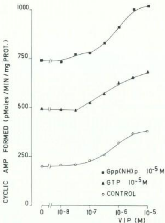
Fig.2. Dose-response curves of VIP-stimulated adenylate cyclase activity of a guinea pig brain synaptosomal fraction in absence ( \circ — \circ ) and presence of 10^{-5} M GTP ( \blacktriangle — \blacktriangle ) or 10^{-5} M Gpp(NH)p ( \blacksquare — \blacksquare ). The results obtained in the standard assay conditions (7 min incubation at 37°C) are the mean of three experiments.
