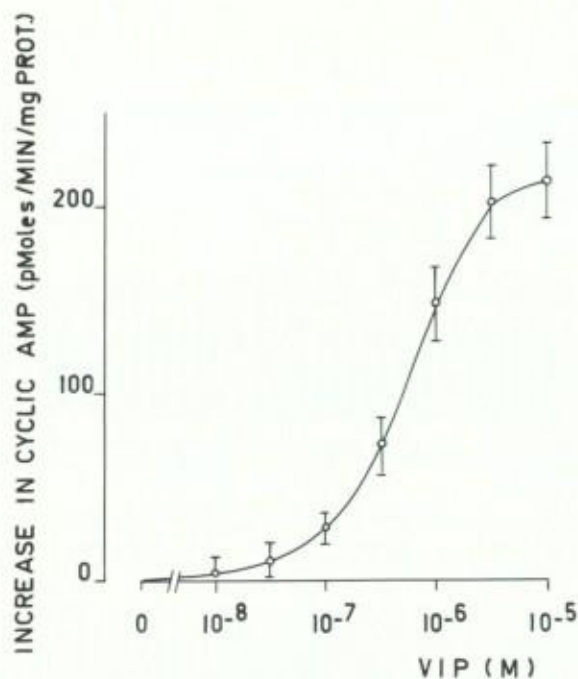
Fig.1. Dose-response curve of adenylate cyclase activation of a guinea pig brain synaptosomal fraction in presence of increasing concentrations of VIP. The results obtained in the standard assay conditions (7 min incubation at 37°C) are presented as increases in cyclic AMP over the basal value ( 189 \pm 12 pmol/min/mg protein) and are the mean \pm SEM of 6 determinations.
