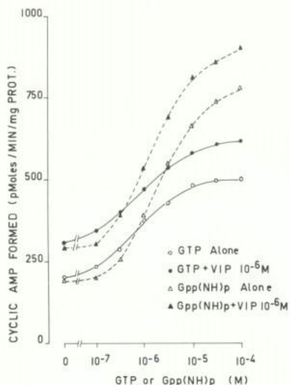
Fig. 3. Dose-response curves of guanyl triphosphate nucleotide-stimulated adenylate cyclase activity of a guinea pig synaptosomal fraction in absence (open symbols) or presence (closed symbols) of 10^{-6} M VIP. The results for GTP ( \circ, \bullet ) and Gpp(NH)p ( \triangle, \blacktriangle ) are the mean of three experiments.
