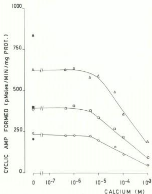
Fig. 4. Effect of 0.5 mM EGTA (closed symbols) and increasing concentrations of calcium (open symbols) on basal ( \circ, \bullet ); 3.10^{-6} M VIP ( \square, \blacksquare ); and 3.10^{-5} M Gpp(NH)p ( \triangle, \blacktriangle ) stimulated adenylate cyclase of a guinea pig brain synaptosomal fraction. The results are the mean of three experiments.
