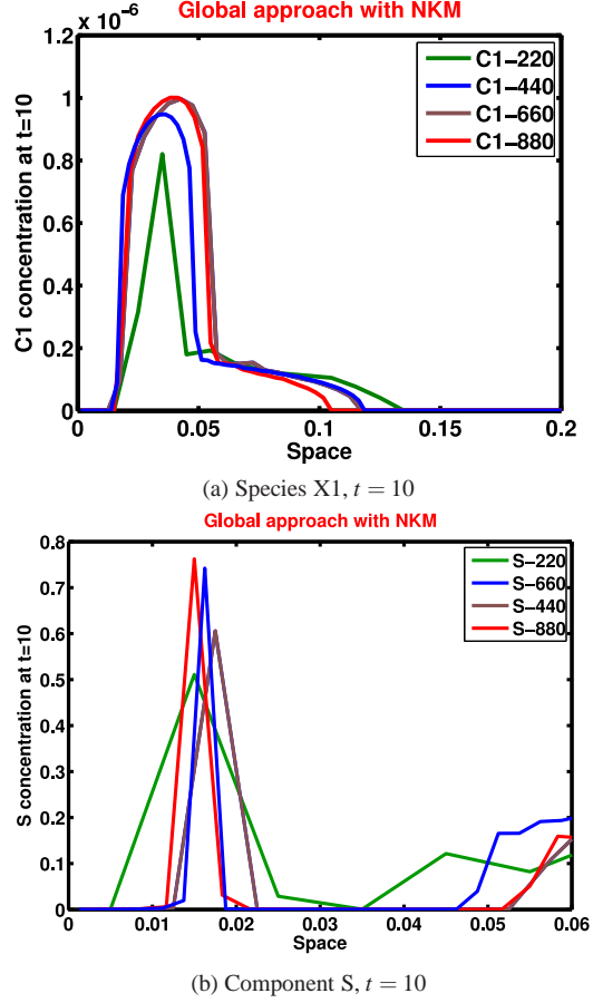
Fig. 7: Concentration profiles
