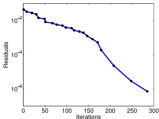
Fig. 8: Iterations
