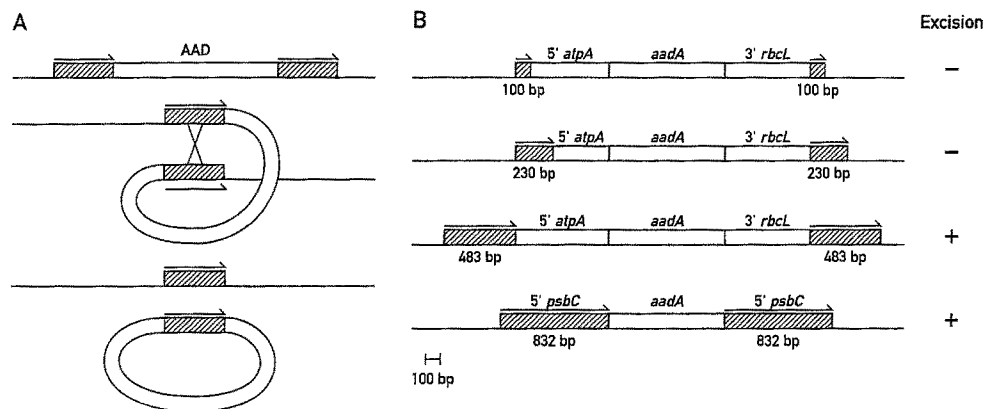
Fig. 1A Excision of aadA by homologous recombination. A homologous recombination event between two direct repeats (hatched bars and arrows) leads to the excision of the selectable marker aadA (open bar). B Structure of the various constructs containing the aadA cassette flanked by two direct repeats. The 100- and 230-bp repeats are part of the atpA promoter; the 483-bp repeat originates from the pACYC184 plasmid. The 832-bp repeat includes the psbC promoter and 5' UTR; this promoter in the first repeat drives aadA expression.
