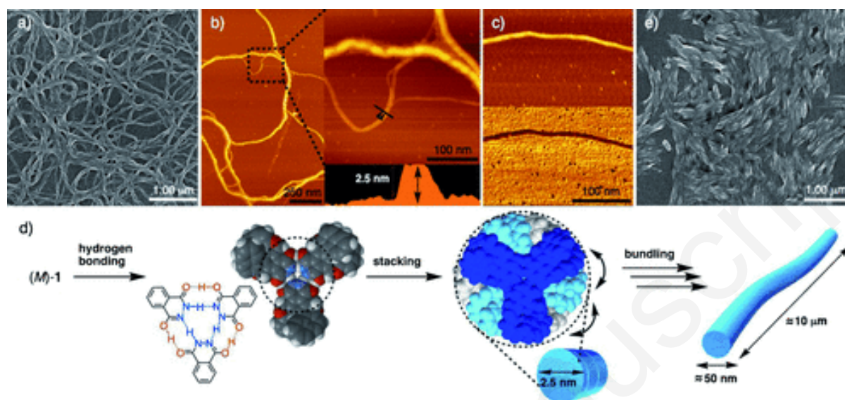
Fig. 12. AFM (b, c) and SEM images of ( M )- 34 (a) and ( rac )- 34 (e) prepared in toluene solutions. d) Postulated mechanism for the formation of supramolecular chiral aggregates from a trimeric association. Reproduced with permission. 32 Copyright 2011, Wiley.
