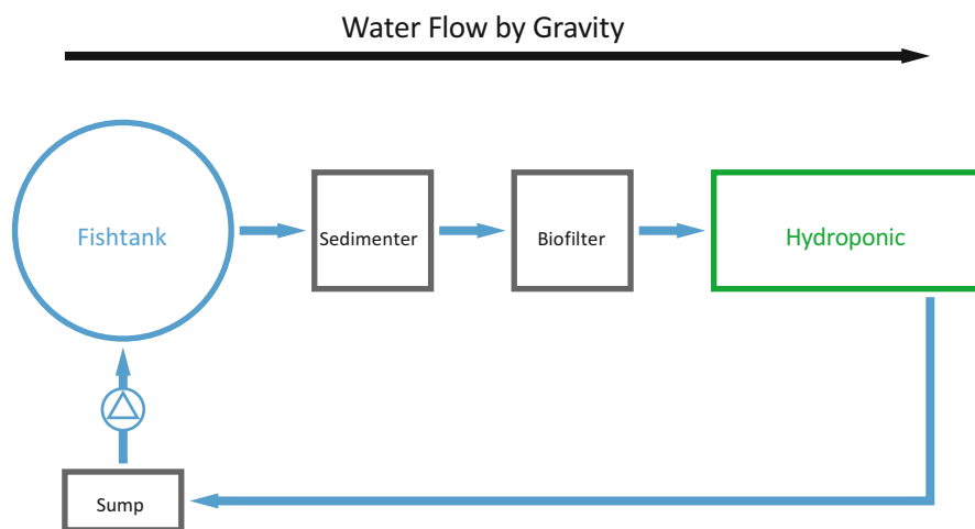
Fig. 7.3 Basic technical system design of a coupled aquaponic system with fish tank, sediment, biofilter, hydroponic unit and a sump where the water is pumped or airlifted back to the fish tanks and flows by gravity along the components
