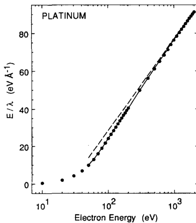
Figure 12. Fano plot for Pt; see caption to Fig. 11.
