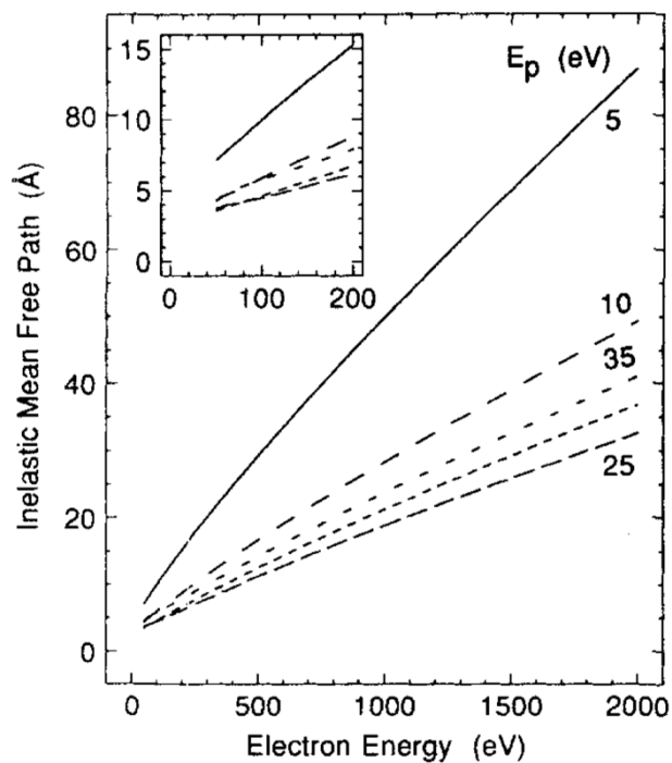
Figure 27. Plots of IMFP versus energy for Al (with E_p = 15.8 eV) from TPP-2 (curve adjacent to the bottom curve) and of evaluations of TPP-2 with Al parameters except that the free-electron plasmon energy E_p was varied as shown.
