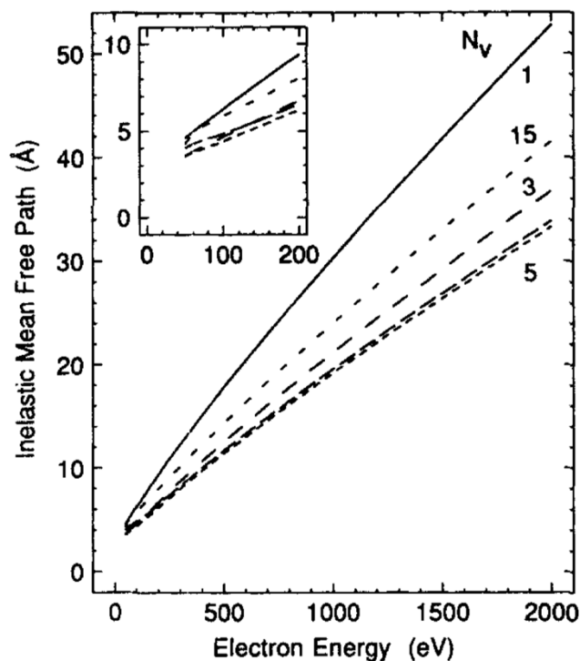
Figure 26. Plots of IMF versus energy for Al from TPP-2 (curve with N_v = 3 ) and of evaluations of TPP-2 with Al parameters except that the number of electrons per atom N_v was varied as shown. The curve adjacent to the bottom N_v = 5 curve is for N_v = 10 .
