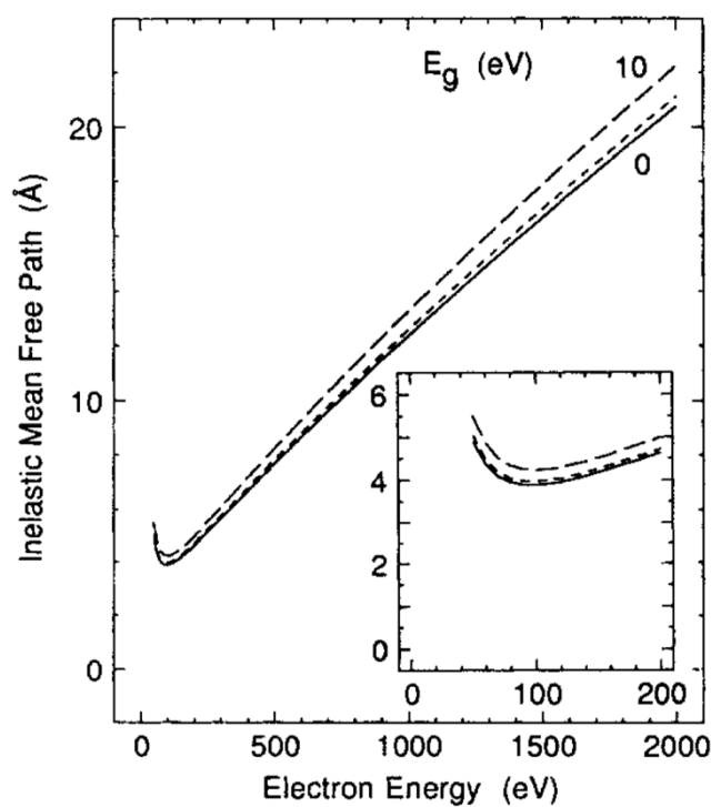
Figure 32. Plots of IMFP versus energy for Au from TPP-2 (solid line) and of evaluations of TPP-2 with Au parameters except that the band-gap energy E_g was varied. The intermediate curve is for E_g = 5 eV.
