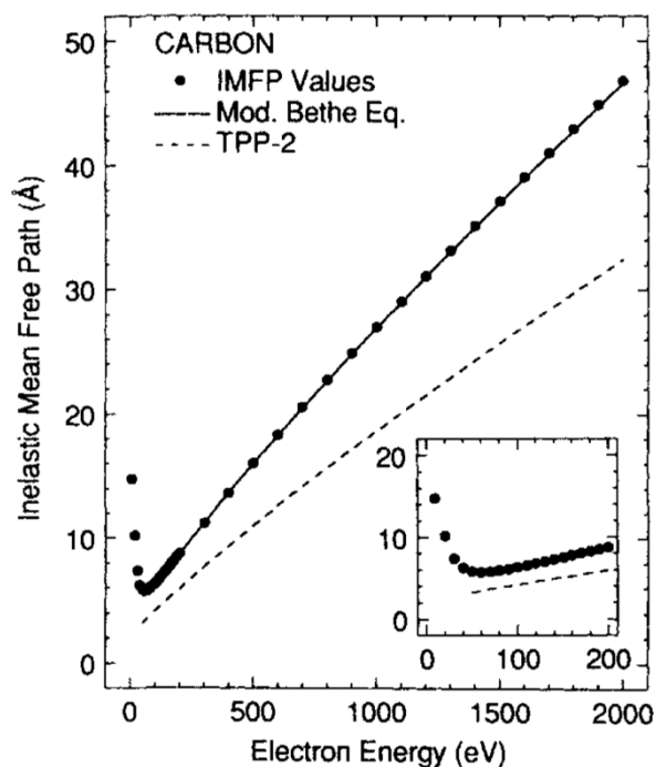
Figure 1. IMFP values (solid circles) calculated for glassy carbon (Table 2) as a function of electron energy. IMFP values are shown for 10 - 40 eV electrons to illustrate trends but these results are not considered to be reliable (see text). The solid line is a fit to the IMFP values with the modified Bethe equation (Eqn. (2)); values of the parameters found in the fit are listed in Table 3. The dashed line shows IMFP values calculated from our predictive formula TPP-2 (Eqn. (2)), where values of the four parameters were calculated from property data for carbon using Eqn. (3). The inset shows the low-energy region on an expanded energy scale.
