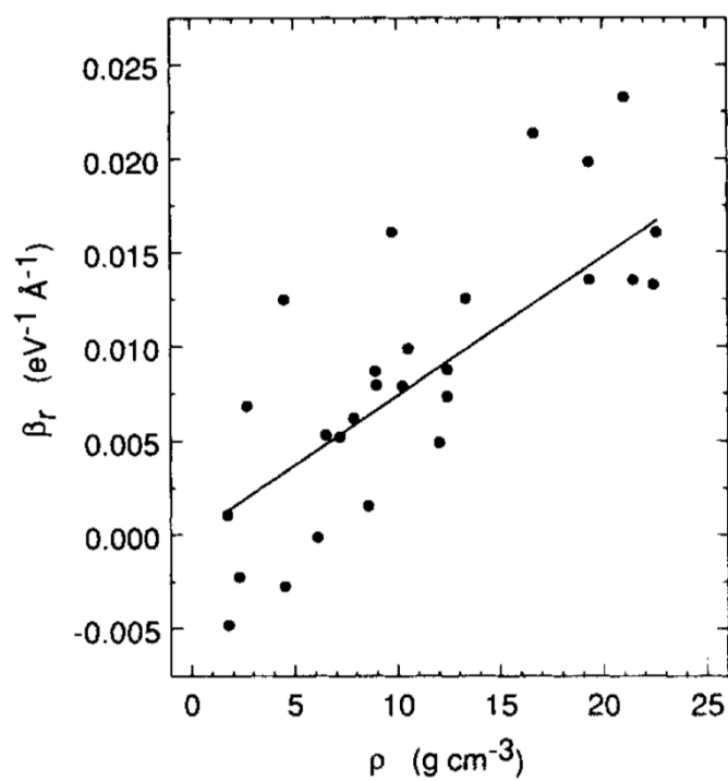
Figure 14. Plot of 11, defined by Eqn. (4) as a function of density \rho . The solid line shows the line \beta_r = 7.39 \times 10^{-4} \rho .
