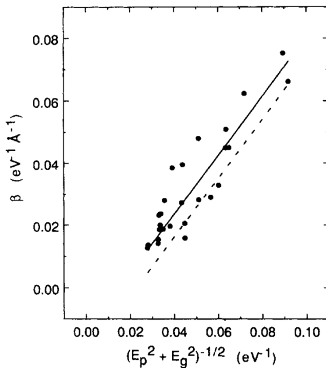
Figure 13. Values of 11 (solid circles) found for each element (Table 3) from the fits of Eqn. (2) to the calculated IMFPs (Table 2) plotted versus (E_p^2 + E_g^2)^{-1/2} . The dashed line is a plot of [0.944 (E_p^2 + E_g^2)^{-1/2} - 0.0216] while the solid line shows a plot of Eqn. (3a) for \rho = 10 \text{ g cm}^{-3} .
