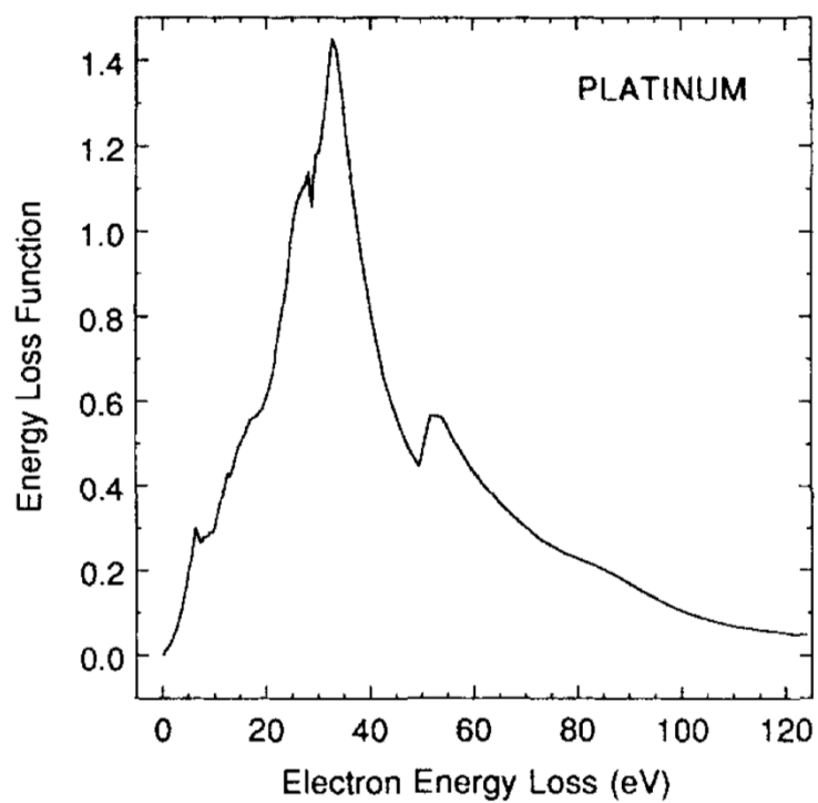
Figure 21. Plot of the electron energy-loss function for \text{Im}[-1/\varepsilon(\omega)] , as a function of energy loss \hbar\omega (Ref. 11).
