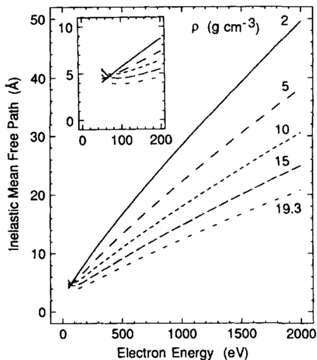
Figure 29. Plots of IMFP versus energy for Au from TPP-2 (lowest curve) and of evaluations of TPP-2 with Au parameters except that the bulk density \rho was varied as indicated.
