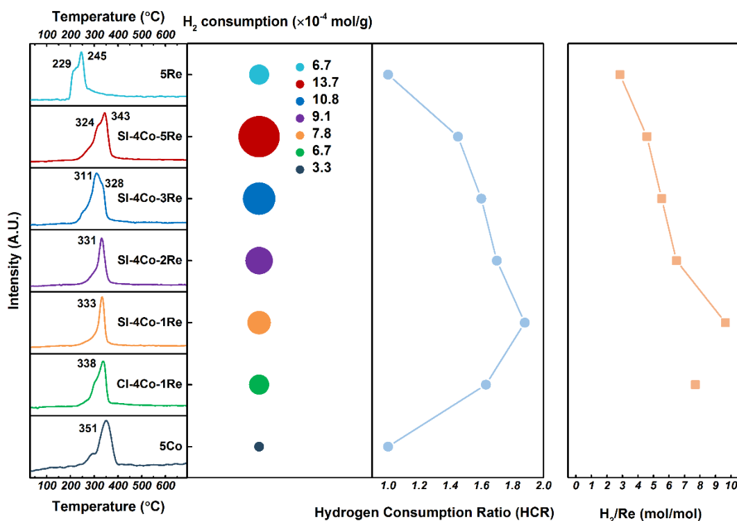
Figure S1. H 2 -TPR results of SI-4Co-XRe/TiO 2 , Cl-4Co-1Re/TiO 2 , 5Co/TiO 2 and 5Re/TiO 2 .
