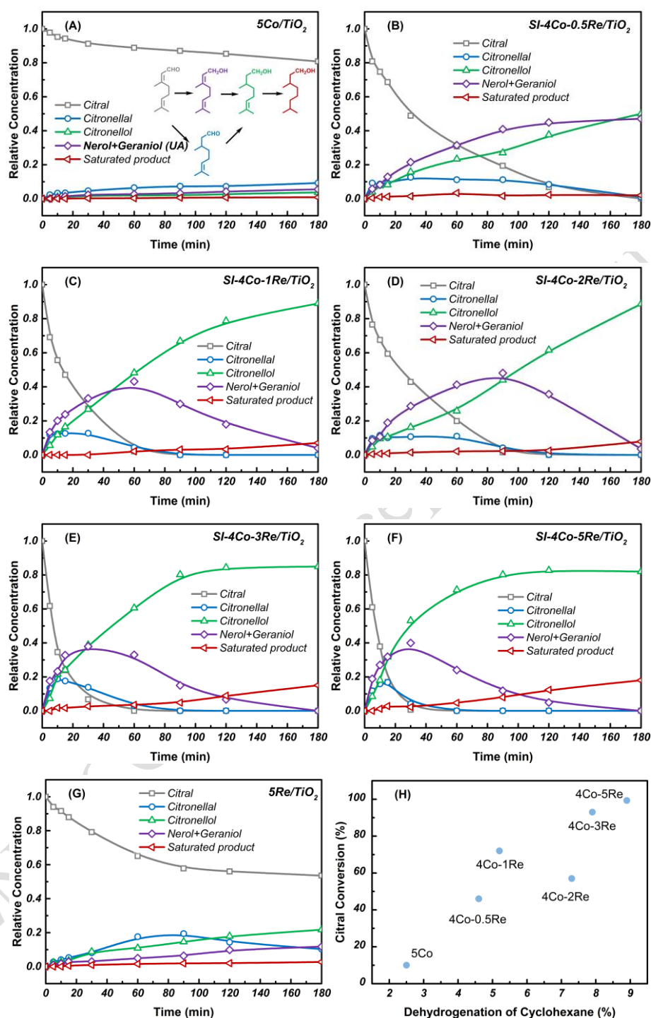
Figure 7. Citral hydrogenation on monometallic Co, Re and SI bimetallic catalysts. (Reaction conditions: 70 °C, 0.4 g catalyst, 100 mL solution (3 mL citral), 75 bar \text{H}_2 )
