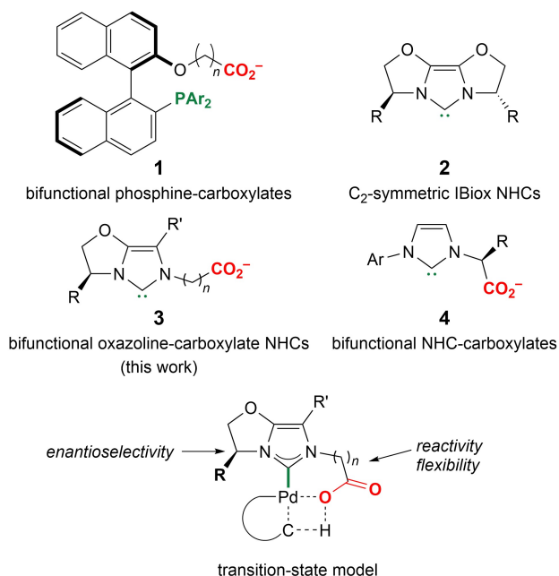
Figure 1. Bifunctional phosphine-carboxylate and NHC-carboxylate ligands.
