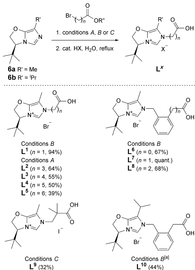
Scheme 2. Synthesis of a library of NHC precursors. Conditions A: alkyl bromide (1.5 equiv.), MeCN, 25 °C, 7 d. Conditions B: alkyl- or benzyl bromide (1.1 equiv.), MeCN, 70 °C, 16 h. Conditions C: alkyl triflate (1.5 equiv.), MeCN, 70 °C, 16 h, then 5 equiv. NaI, acetone, 25 °C, 16 h. [a] 48 h at 70 °C.
