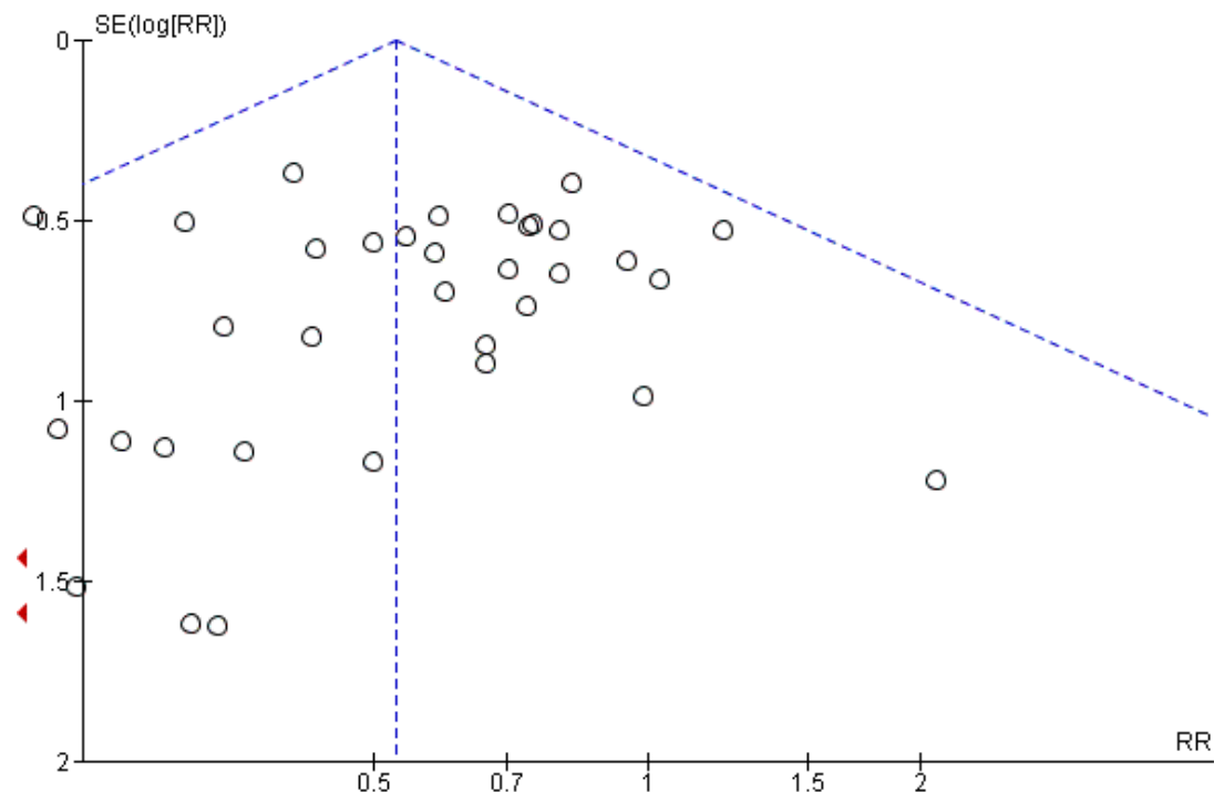
Figure 6. Funnel plot of comparison: I Transobturator (TOR) versus retropubic (RPR) route, outcome: 1.17 Voiding dysfunction
